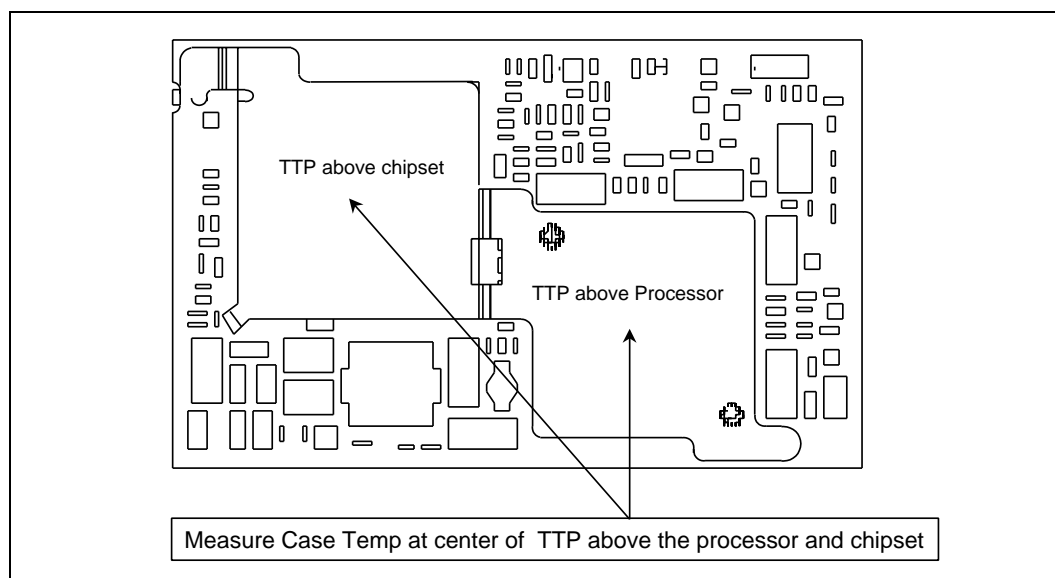
Figure 3. Mounting the Thermocouple
