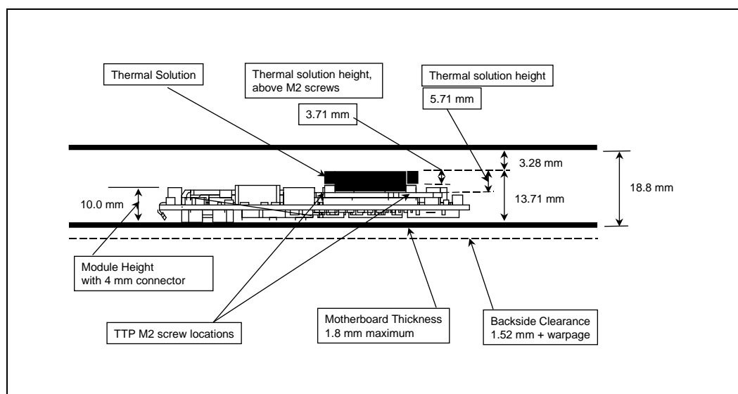
Figure 4. Compact PCI Height Requirements
