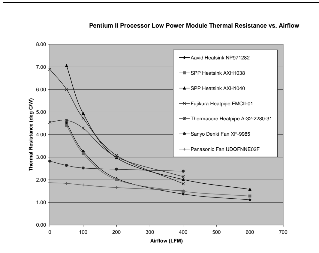
Figure 2. Pentium® II Processor Low Power Module Thermal Resistance vs. Airflow
