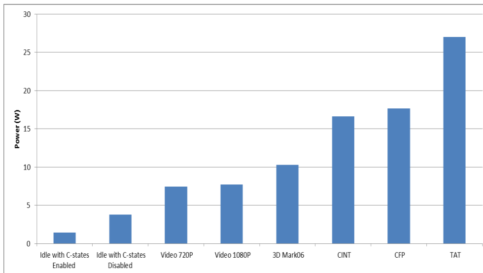
Figure 1. Application Power Guidelines for the Intel® Core™ i5 Processor-3610ME
