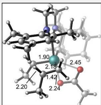
Z-selective olefin metathesis transition state (source K. Houk, UCLA)
