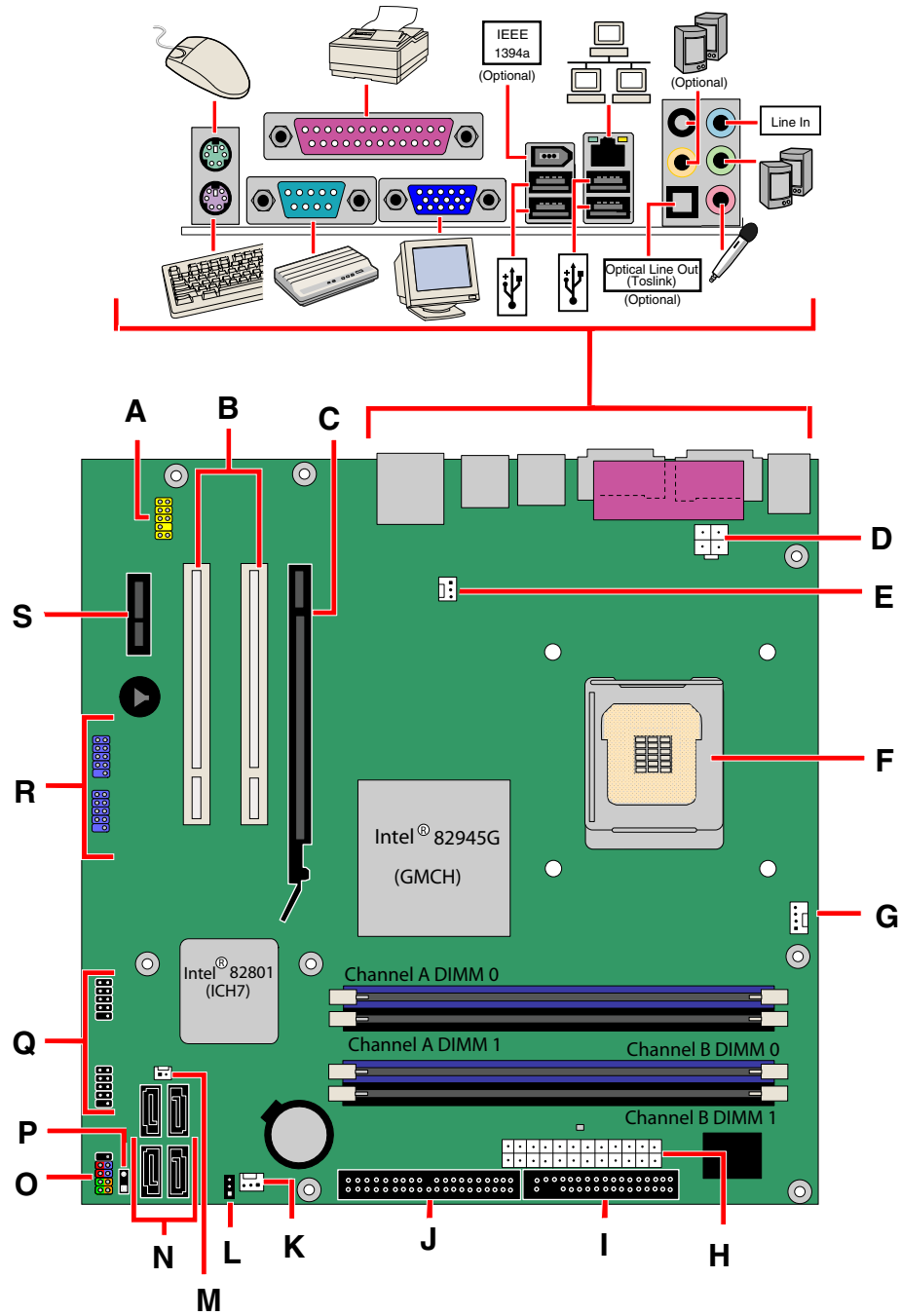
Figure 2. Intel Desktop Board D945GTP Components
