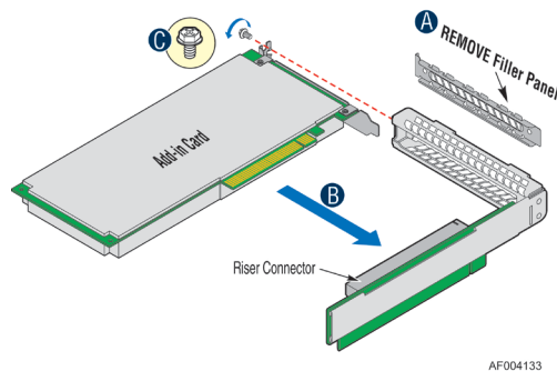
Figure 48. Riser Card Assembly
