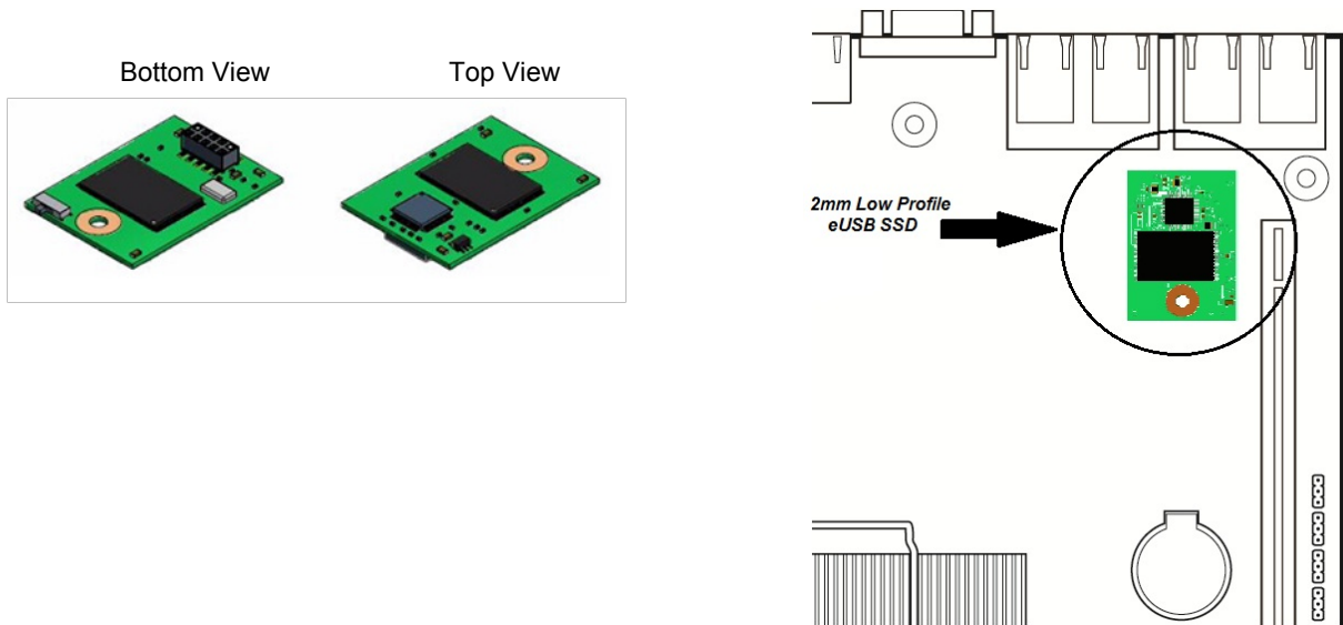
Figure 21. Low Profile eUSB SSD Support
