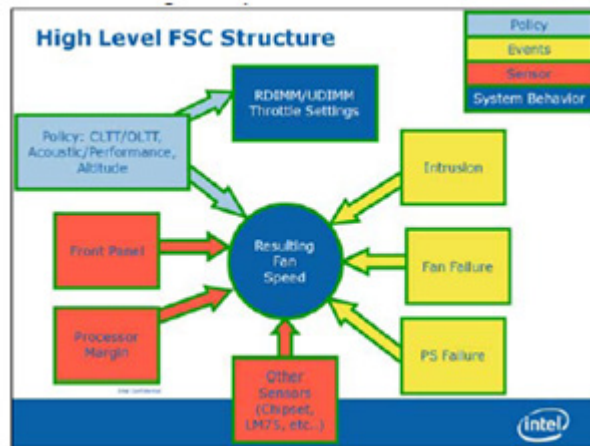
Figure 15. Fan Control Model
