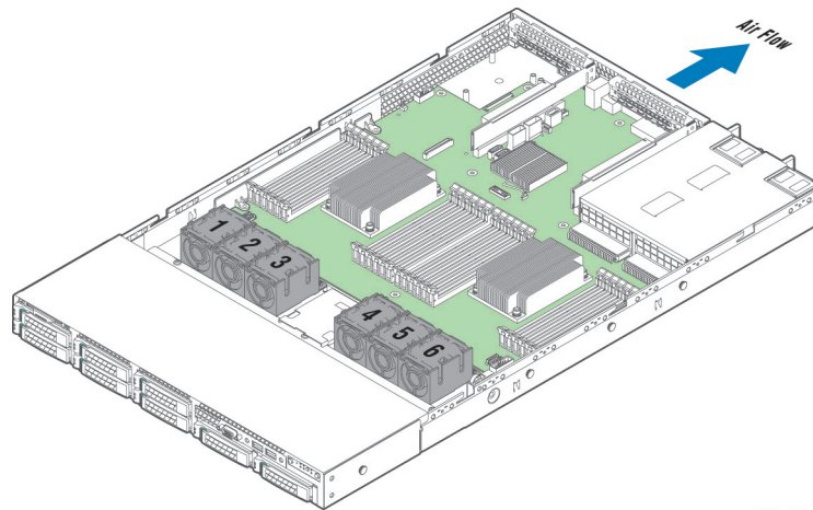
Figure 16. System Fan Identification
