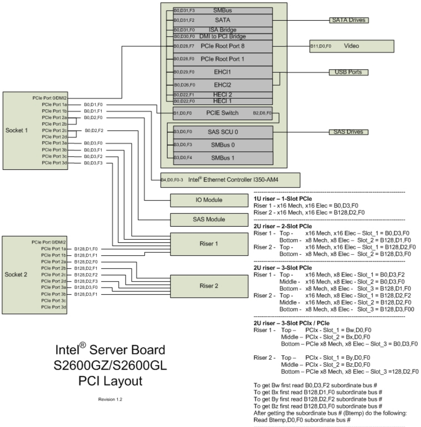
Figure 46. Intel® Server Board S2600GZ/GL PCI Bus Layout Diagram
