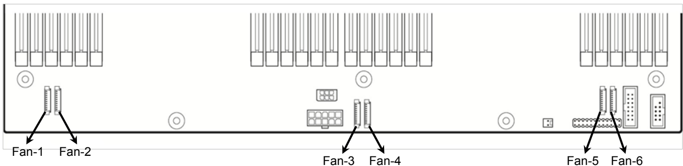
Figure 17. Server Board System Fan Connector Locations
