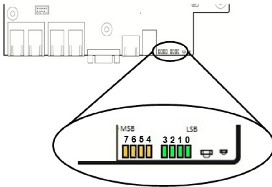
Figure 49. POST Diagnostic LED Location
