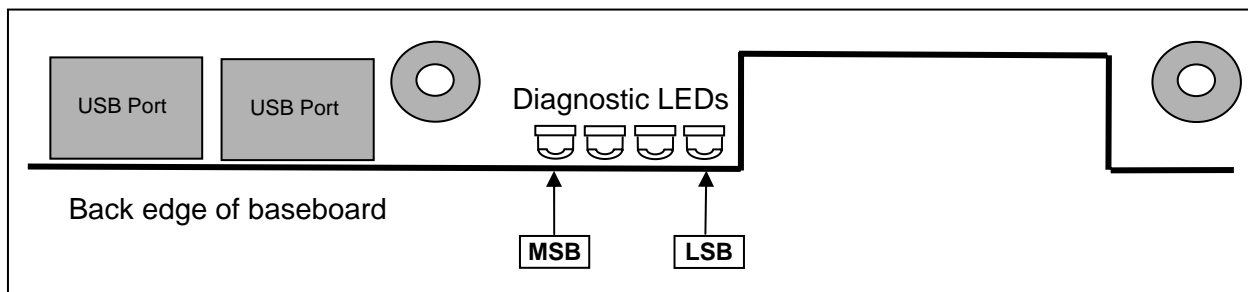
Figure 21. Diagnostic LED Placement Diagram Example
