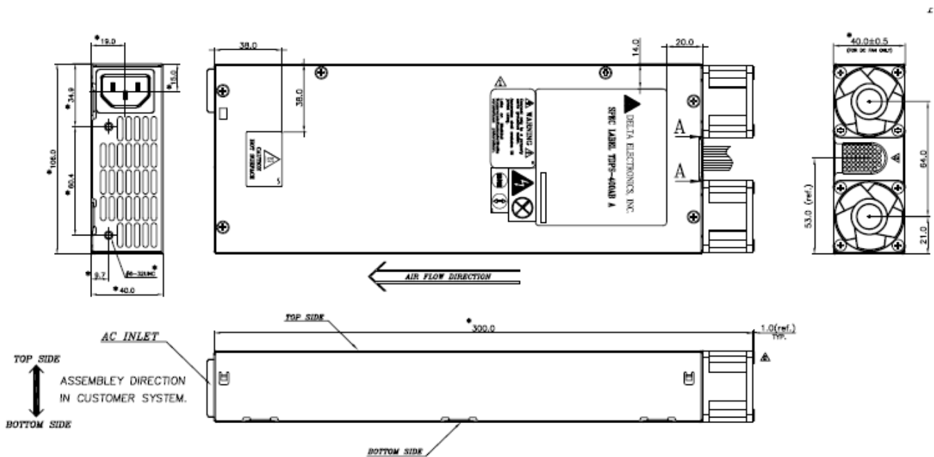
Figure 8. Power Supply Mechanical Drawing
