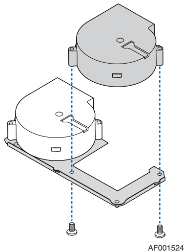
Figure 9. Fan Module Assembly - SR1530CL/SR1530CLR (SATA)
