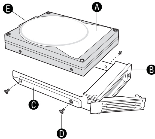
Figure 15. Hard Drive Tray Assembly
