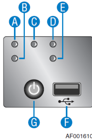
Figure 18. Front Control Panel - SR1530HCL/SR1530HCLR (SATA) and SR1530HCLS/SR1530HCLSR (SAS)
