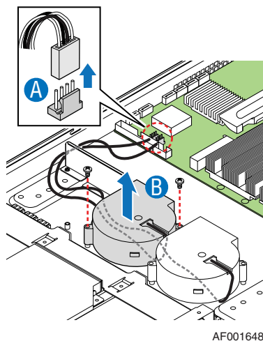
Figure 10. Fan Module Assembly - SR1530HCL/SR1530HCLR (SATA) and SR1530HCLS/SR1530HCLSR (SAS)
