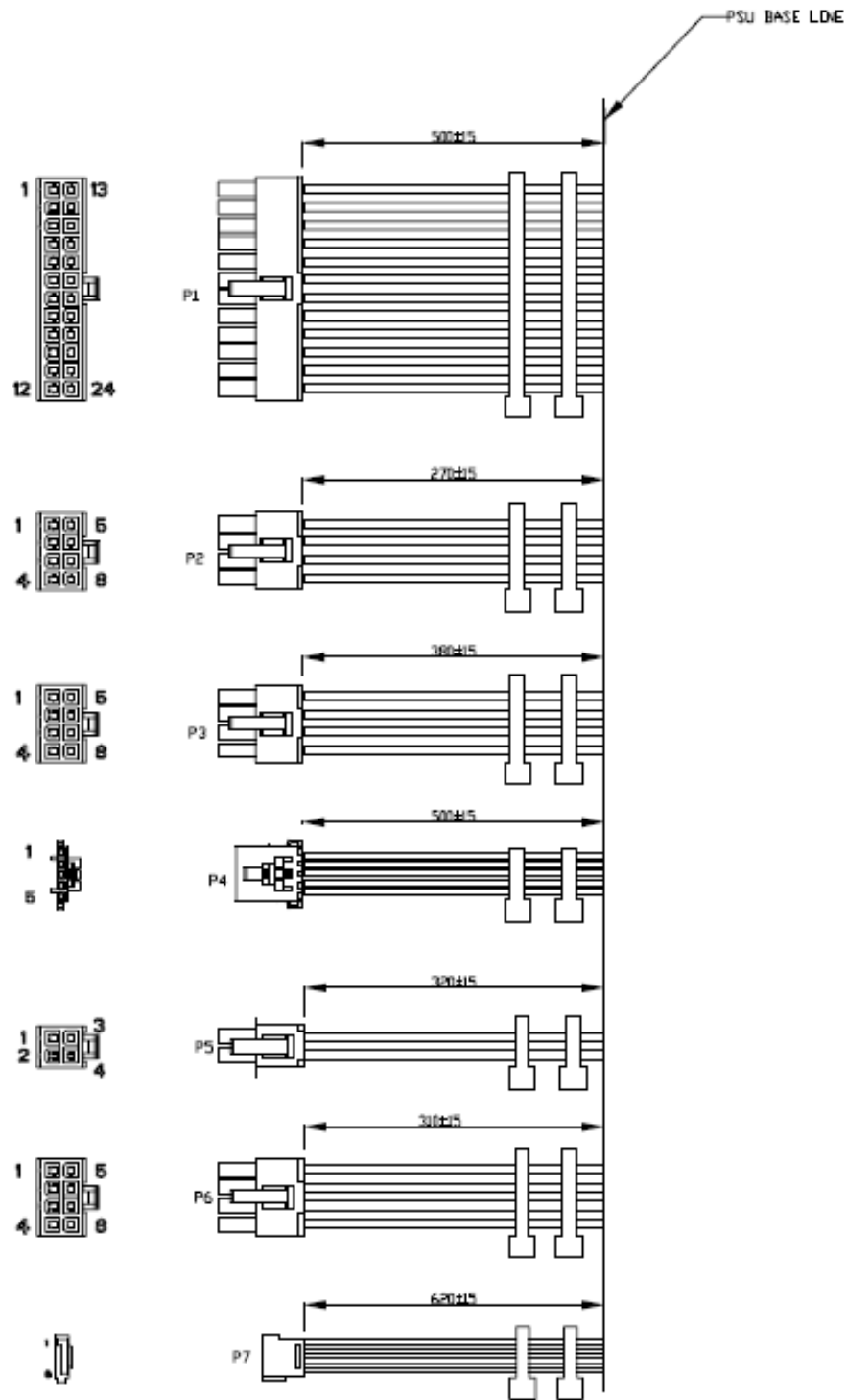
Figure 13. Power Supply Cable Harness
