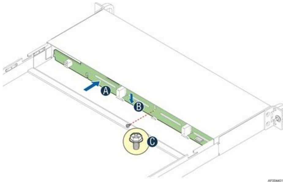
Figure 23. Installing 2.5" Drive Hot-Swap Backplane
