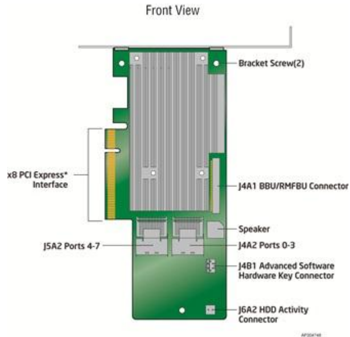
Figure 36. Intel® Integrated RAID Module RMS25PB080 and RMS25PB040
