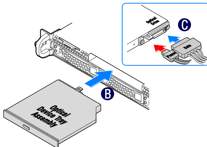
Figure 33. Install a SATA Optical Drive
