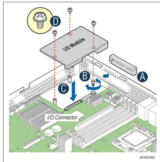
Figure 62. Installing I/O Module
