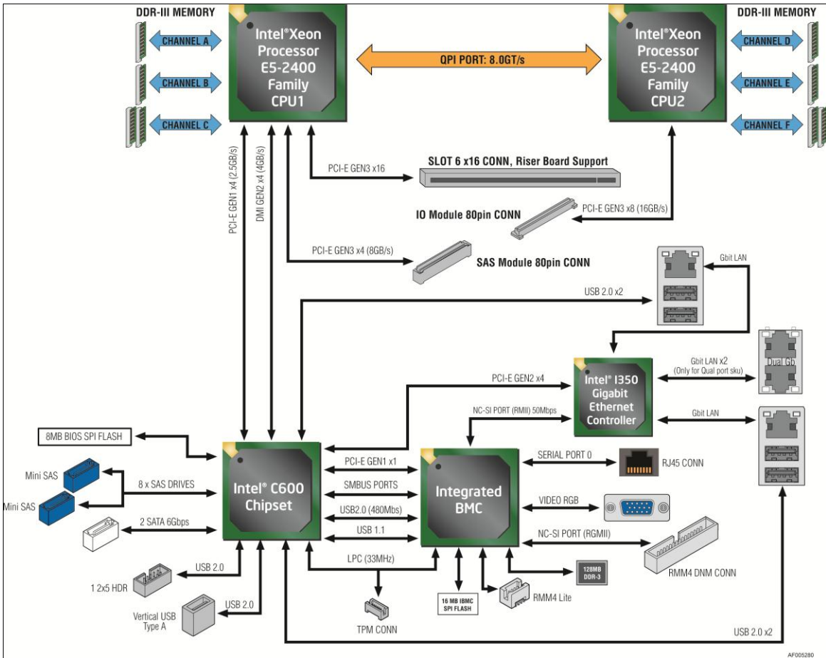
Figure 60. Riser Slot Architecture – Intel® C600 Upgrade Key NOT installed
