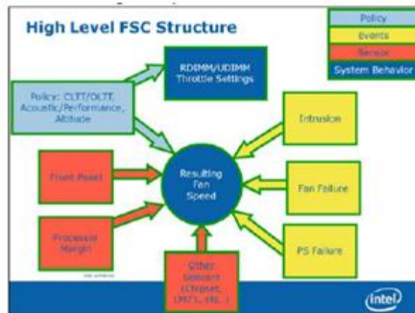
Figure 17. Fan Control Model
