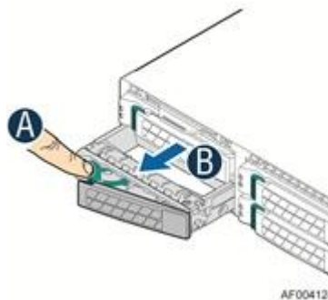
Figure 21. Removing 2.5" Hard Disk Drive
