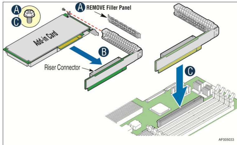
Figure 61. Add-in Card Support
