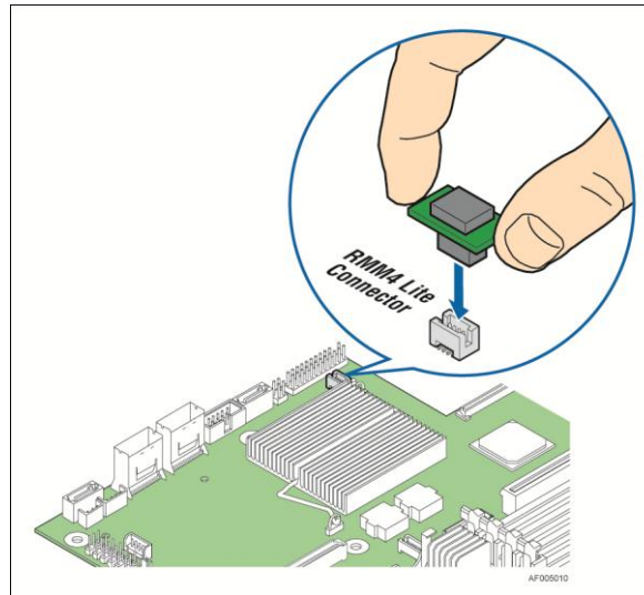
Figure 63. Intel® RMM4 Lite Activation Key Installation
