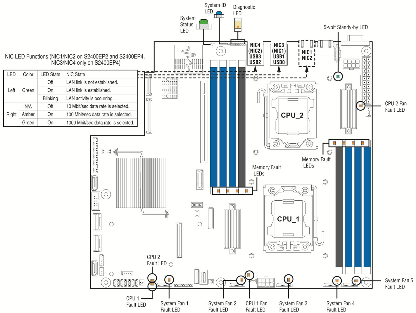
Figure 9. Intel® Light-Guided Diagnostic LEDs - Server Board
