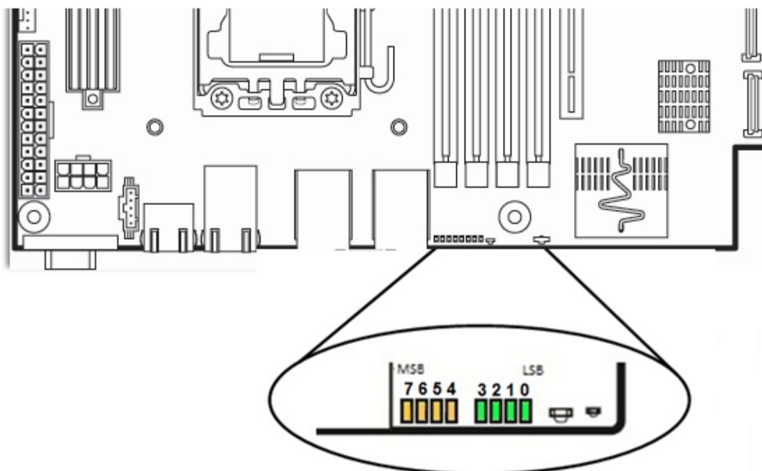
Figure 65. POST Diagnostic LEDs
