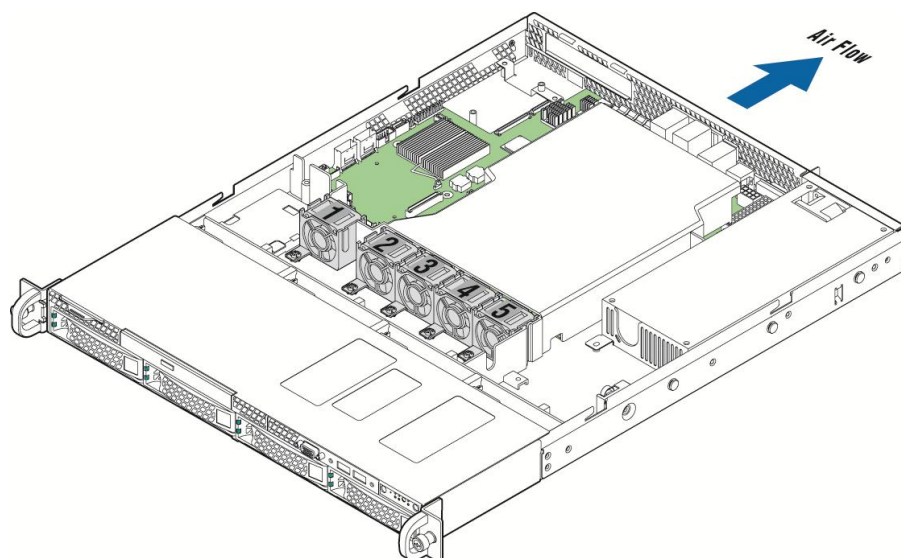
Figure 18. System Fan Identification
