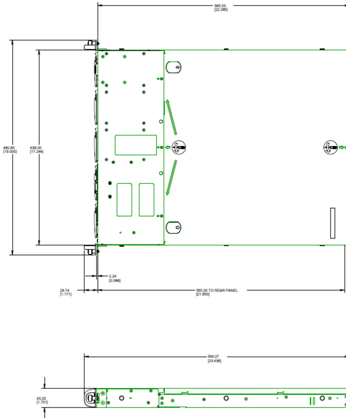
Figure 3. Chassis Dimensions
