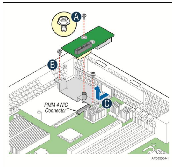
Figure 64. Intel® RMM4 Dedicated Management NIC Installation
