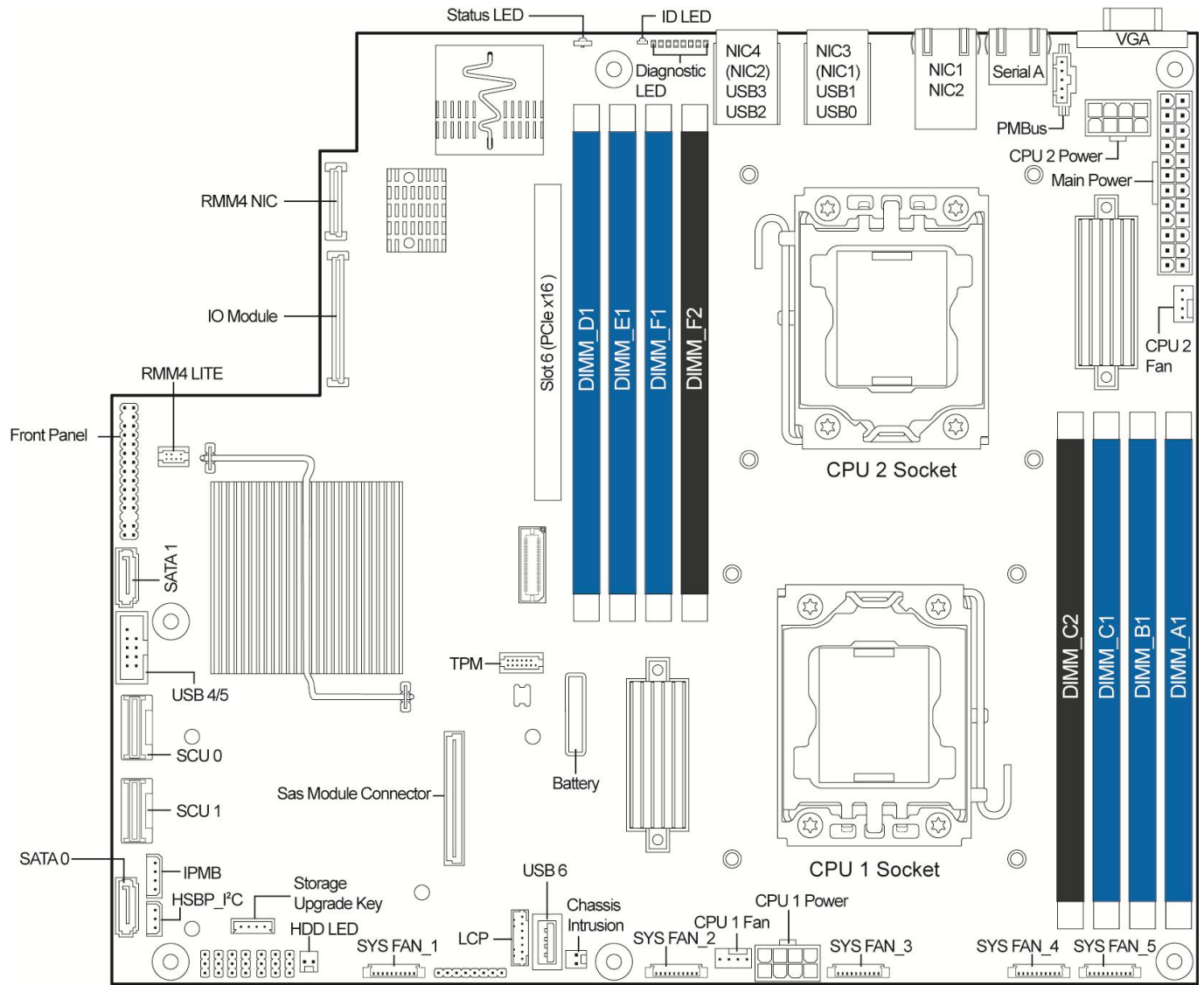
Figure 8. Intel® Server Board S2400EP
