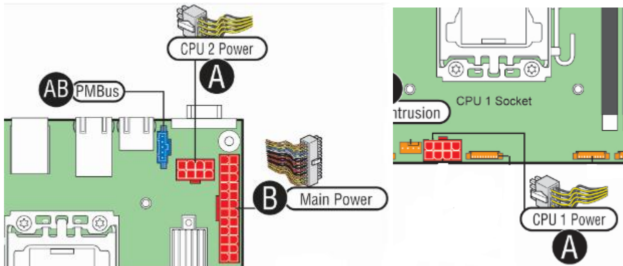
Figure 15. Main Power Connector Identification
