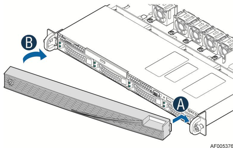
Figure 11. Installing the Optional Front Bezel
