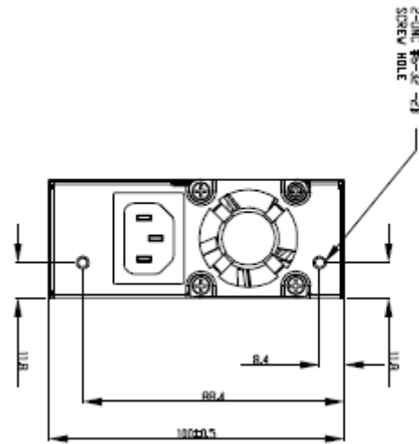
Figure 14. AC and DC Power Supplies - Connector View
