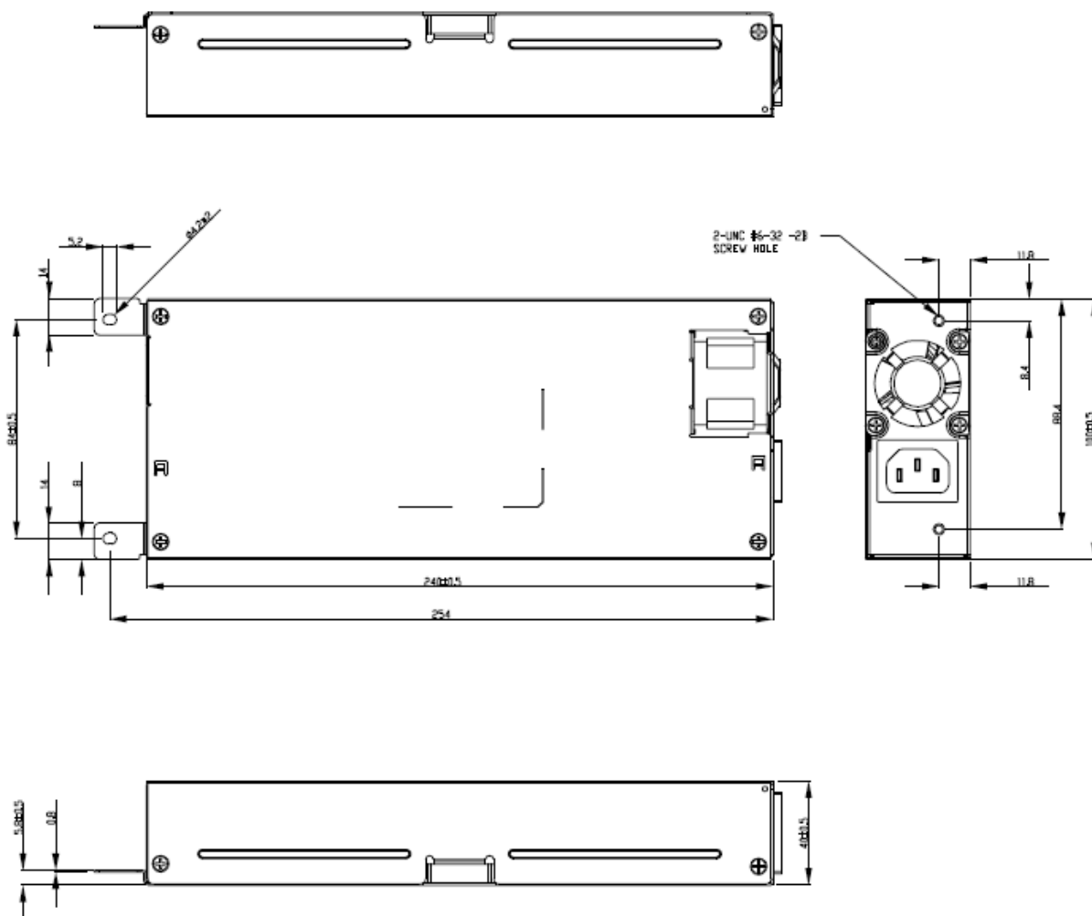
Figure 12. Power Supply Module Mechanical Drawing
