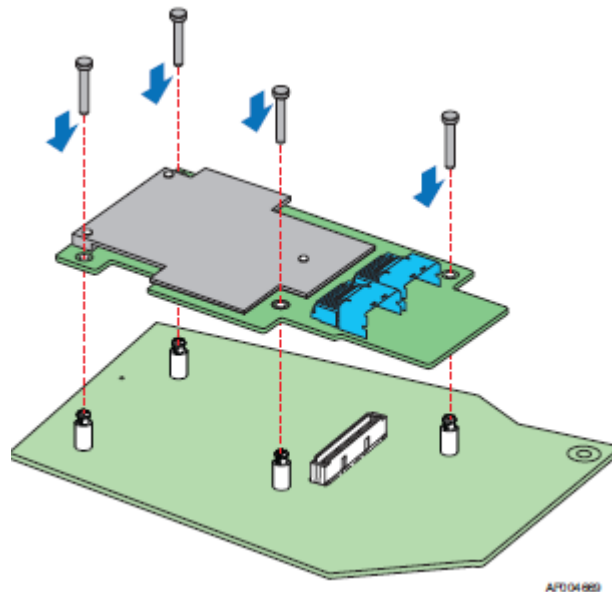
Figure 37. Intel® Integrated RAID Module RMS25JB080 and RMS25JB040
