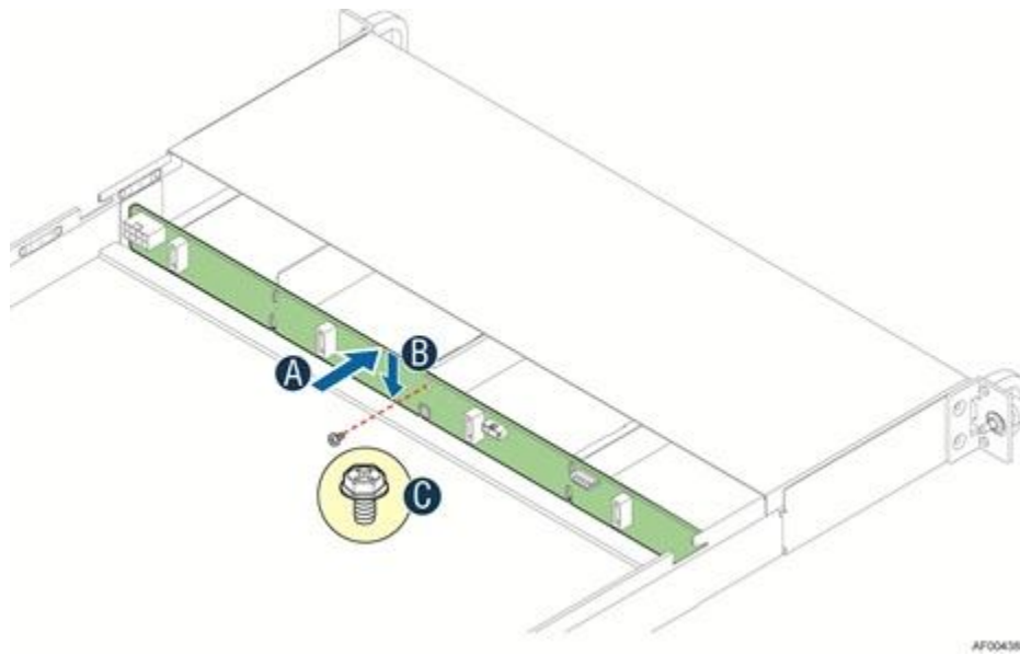
Figure 29. 3.5" Drive Hot-Swap Backplane Installation
