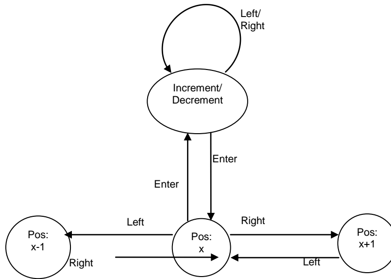
Figure 57. State transition diagram for setting IP Address
