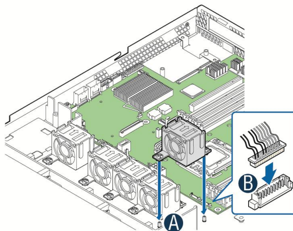
Figure 19. System Fan Assembly
