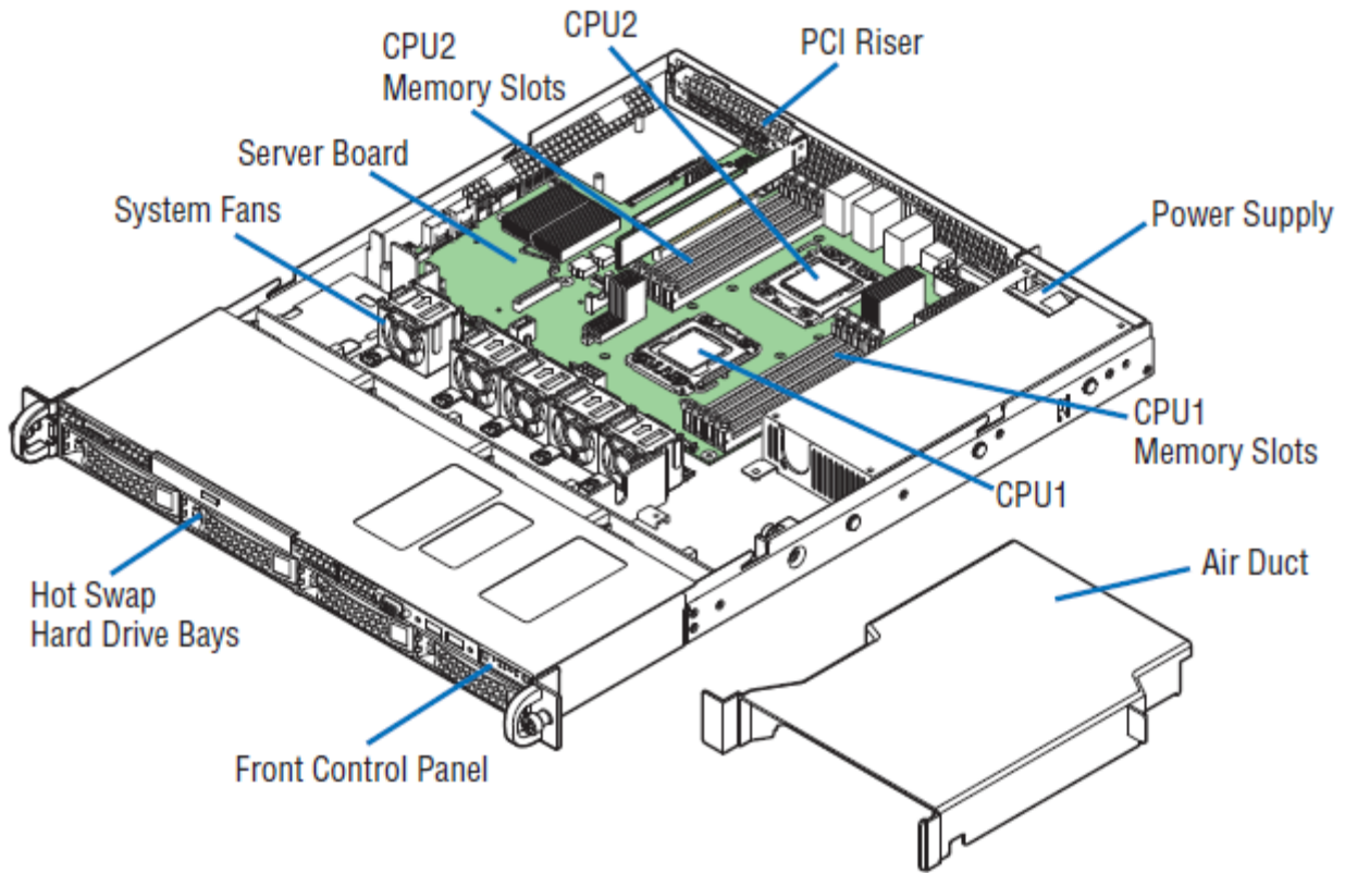
Figure 4. System Components Overview
