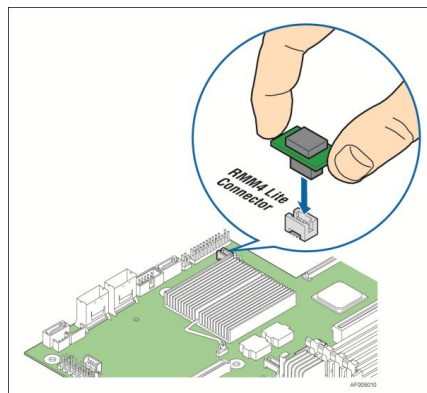
Figure 35. Installing RMM4 Lite Figure
