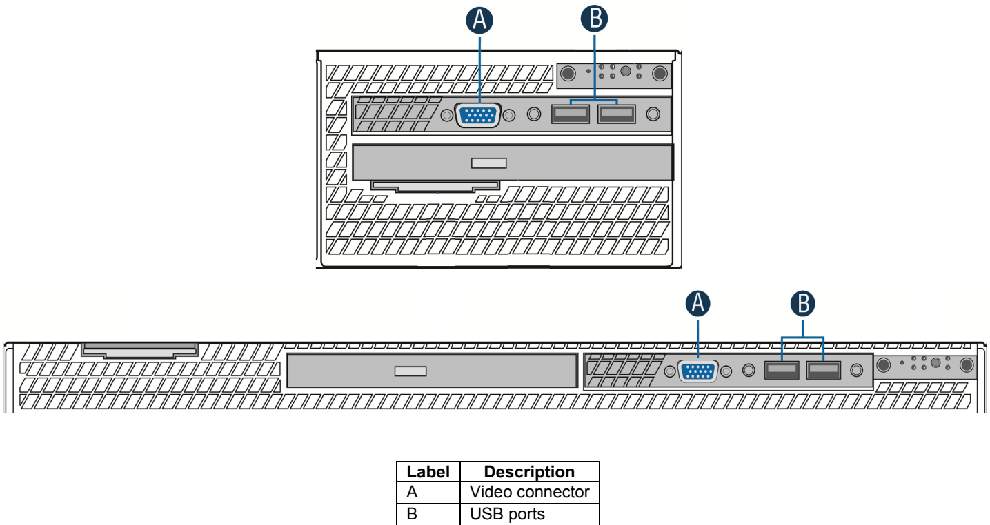
Figure 38. Front I/O Panel Features
