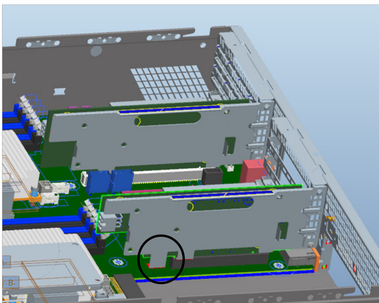
Figure 64. Riser Card #1 Assembly Showing Mechanical Block
