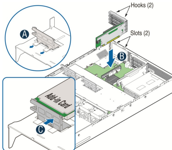
Figure 63. Full Height / Full Length Add-in Card Support
