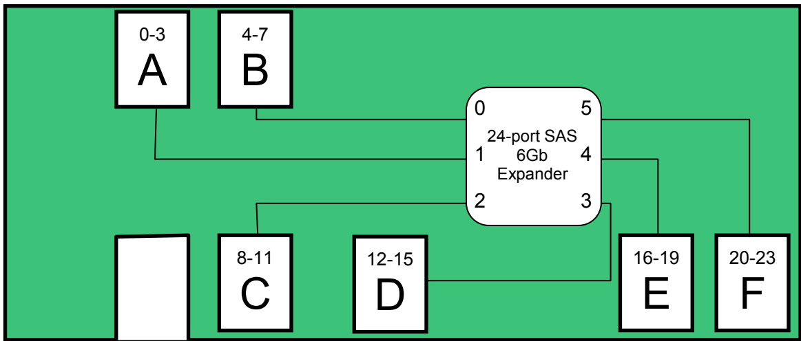
Figure 35. 24-Port Expander SAS Connector/Drive Identification Block Diagram
