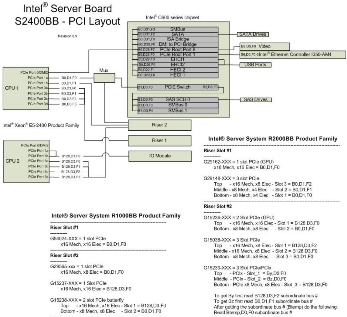
Figure 62. Intel® Server Board S2400BB PCI Bus Layout Diagram
