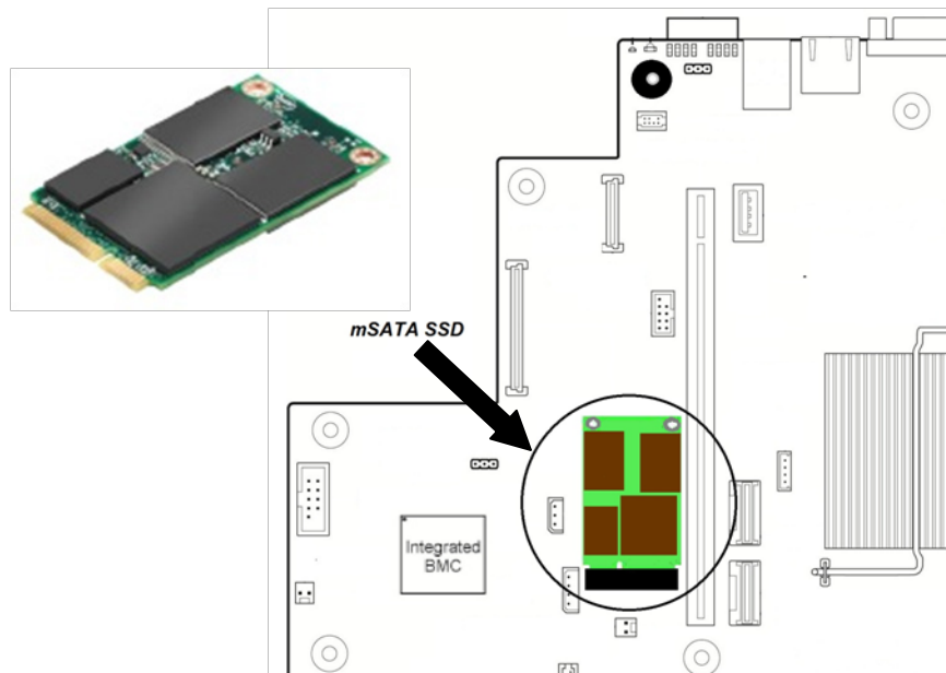
Figure 31. mSATA Placement
