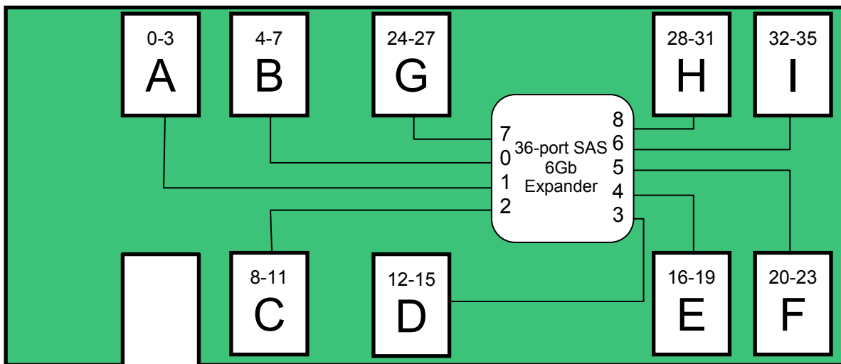
Figure 36. Internal 36-Port SAS Expander Card (RES2CV360)
