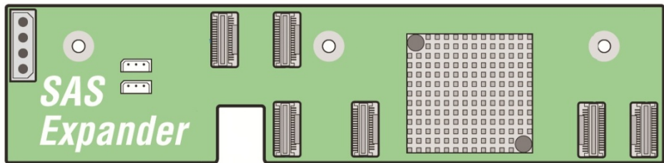
Figure 34. Internal 24-Port SAS Expander Card (RES2CV240)
