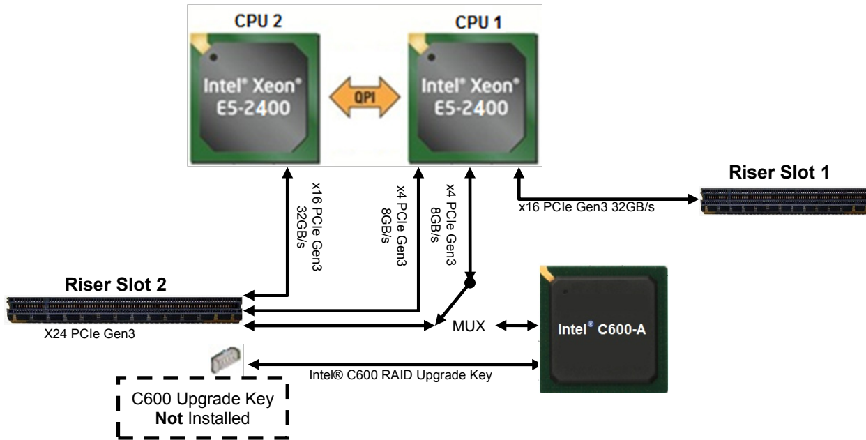
Figure 60. Riser Slot Architecture – Intel® C600 Upgrade Key NOT Installed
