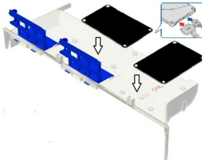
Figure 28. 2.5" Internal Fixed Mount Solid State Drive (SSD) Mounting Option
