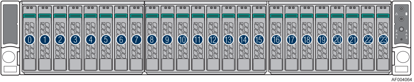
Figure 24. 2.5" Hard Drive Bay - 24 Drive Configuration
