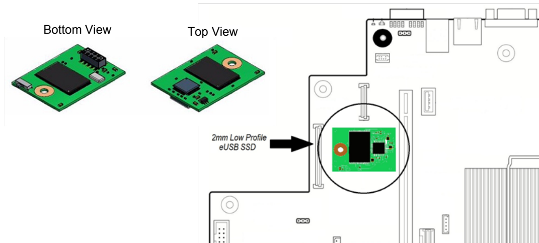
Figure 29. Low Profile eUSB Placement
