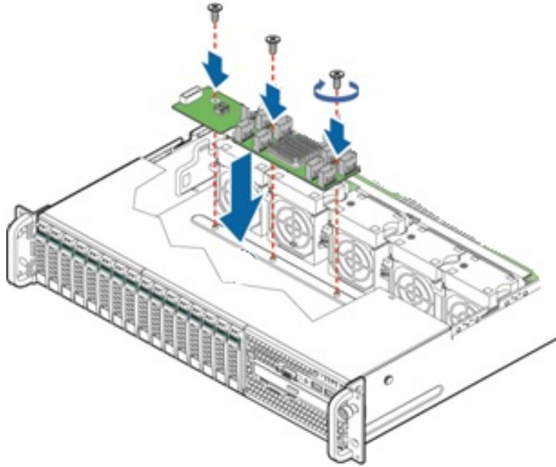
Figure 33. Internal SAS Expander Installation
