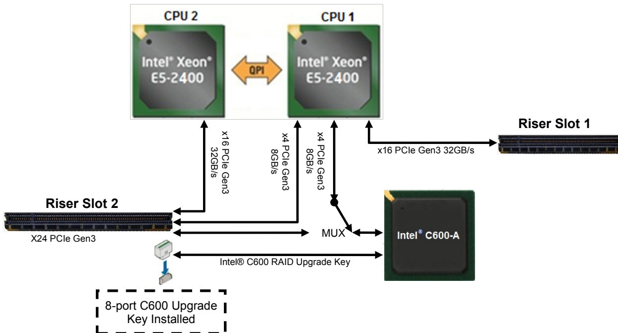
Figure 61. Riser Slot Architecture - Intel® C600 Upgrade Key Installed
