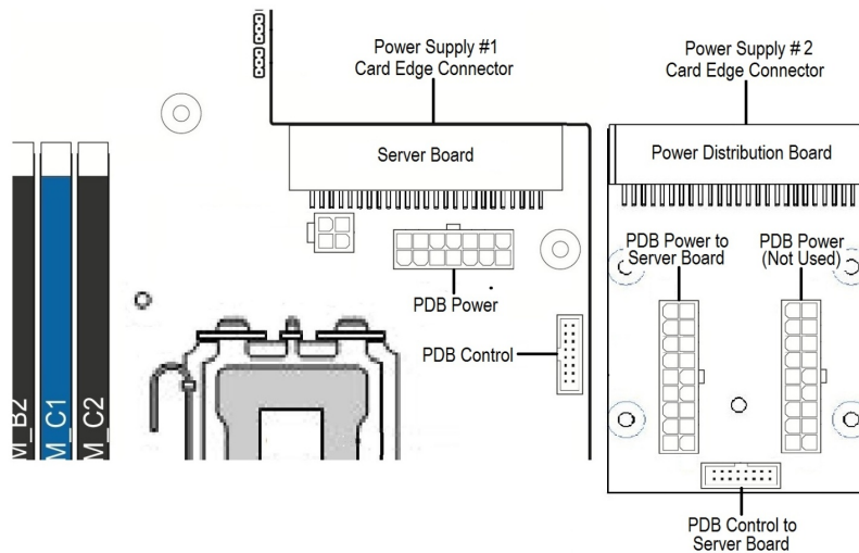
Figure 16. Main Power Connector Identification
