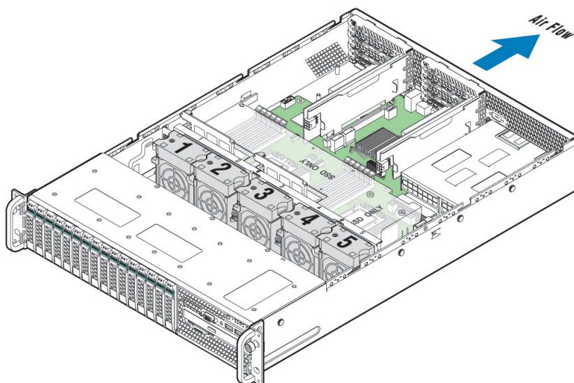
Figure 20. System Fan identification
