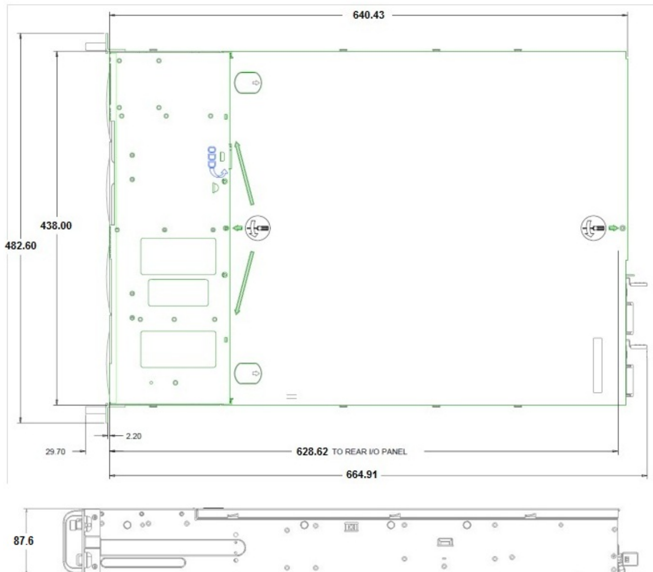
Figure 1. Chassis Dimensions
