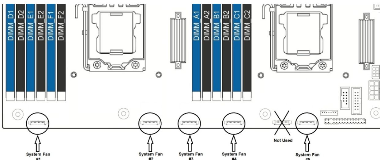
Figure 22. Server Board System Fan Connector Locations
