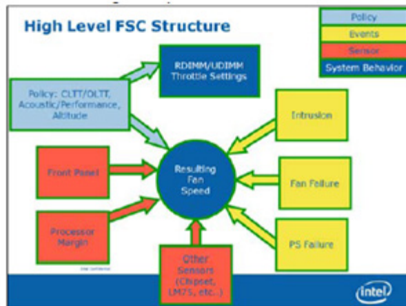
Figure 19. Fan Control Model
