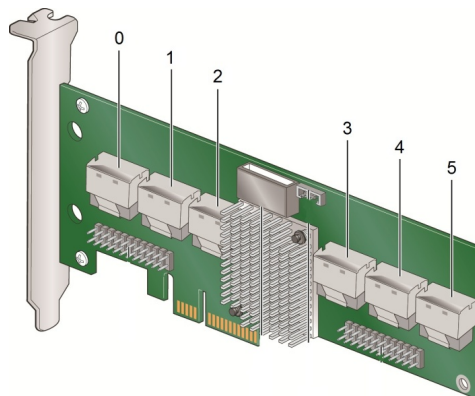
Figure 32. 24 Port PCIe Intel® RAID Expander Card RES2SV240
