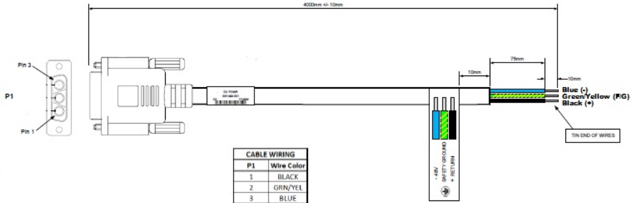
Figure 18. DC Power Cord
