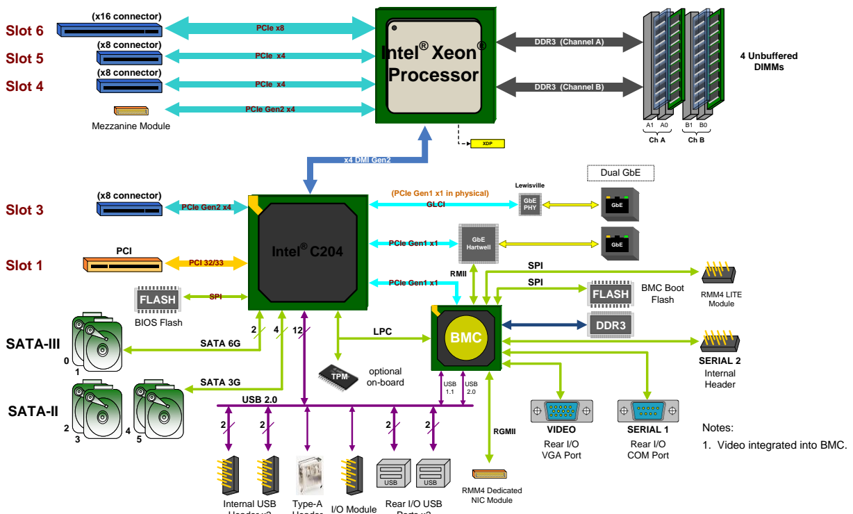
Figure 11. Intel® Server Board S1200BTL Functional Block Diagram
