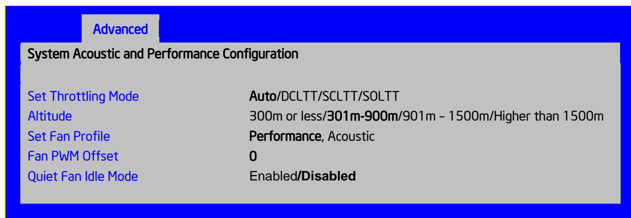
Figure 38. System Acoustic and Performance Configuration
