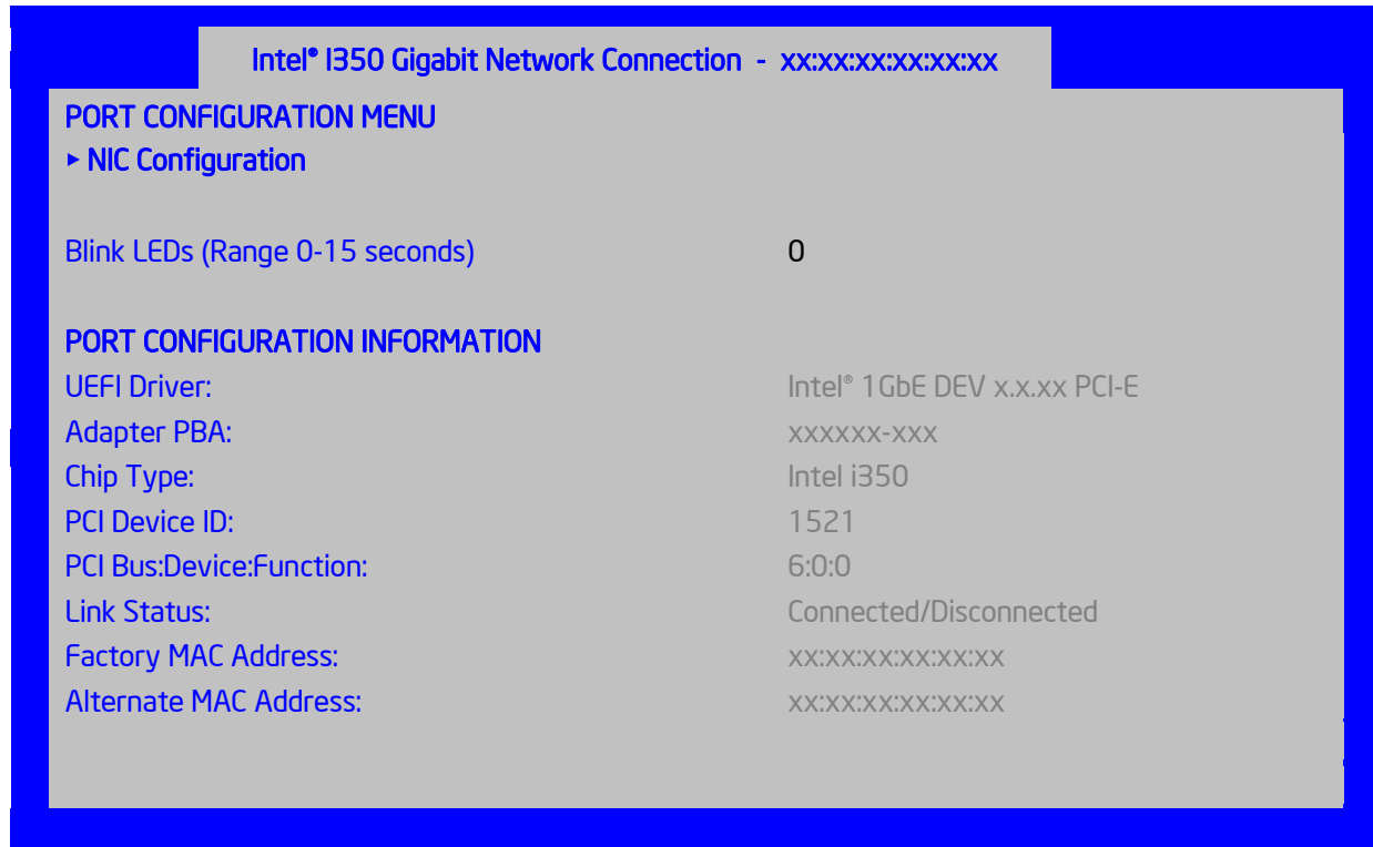
Figure 34. i350 NIC Configuration Screen
