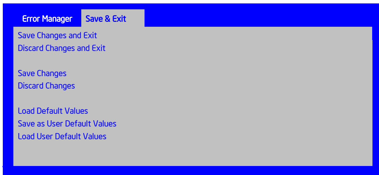
Figure 51. Exit Screen
