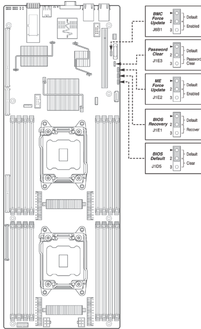
Figure 52. Jumper Blocks (J6B1, J1E2, J1E3, J1E1, J1D5)
