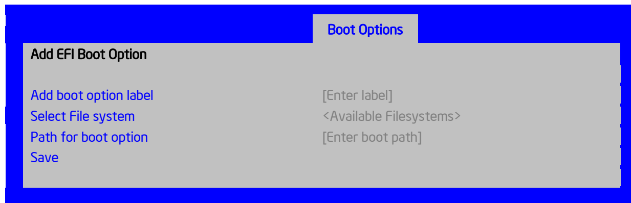
Figure 47. Add EFI Boot Option Screen
