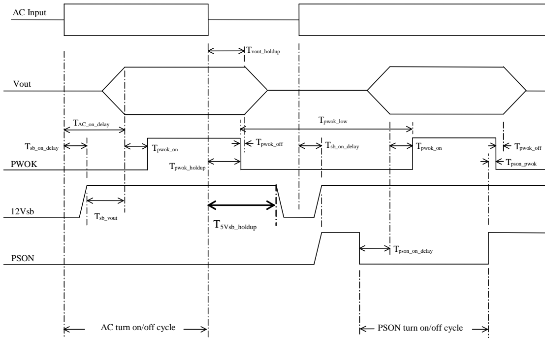
Figure 57. Turn On/Off Timing (Power Supply Signals)
