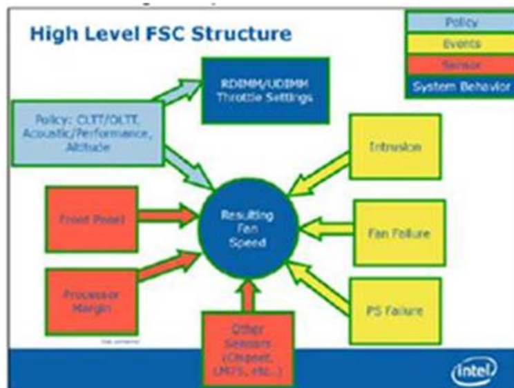
Figure 56. Fan Speed Control Structure
