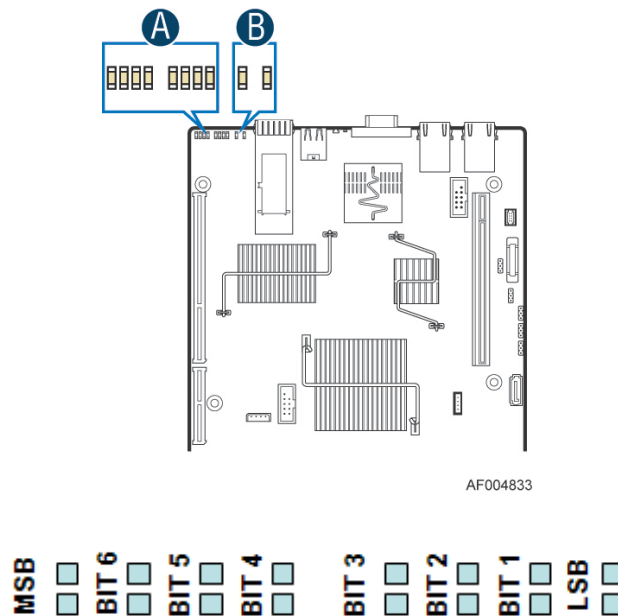
Figure 58. Diagnostic LED Placement Diagram
