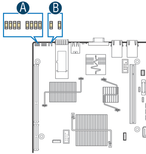
Figure 55. Rear Panel Diagnostic LEDs (Block A)
