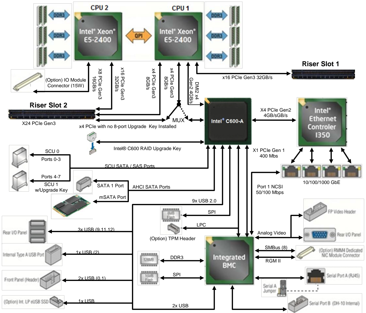
Figure 6. Intel® Server Board S2400BB Functional Block Diagram
