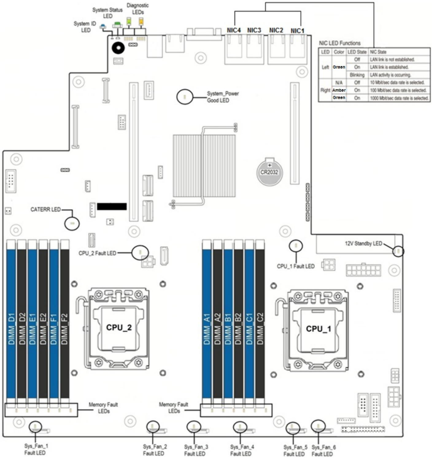
Figure 3. Intel® Light Guided Diagnostic LED Identification
