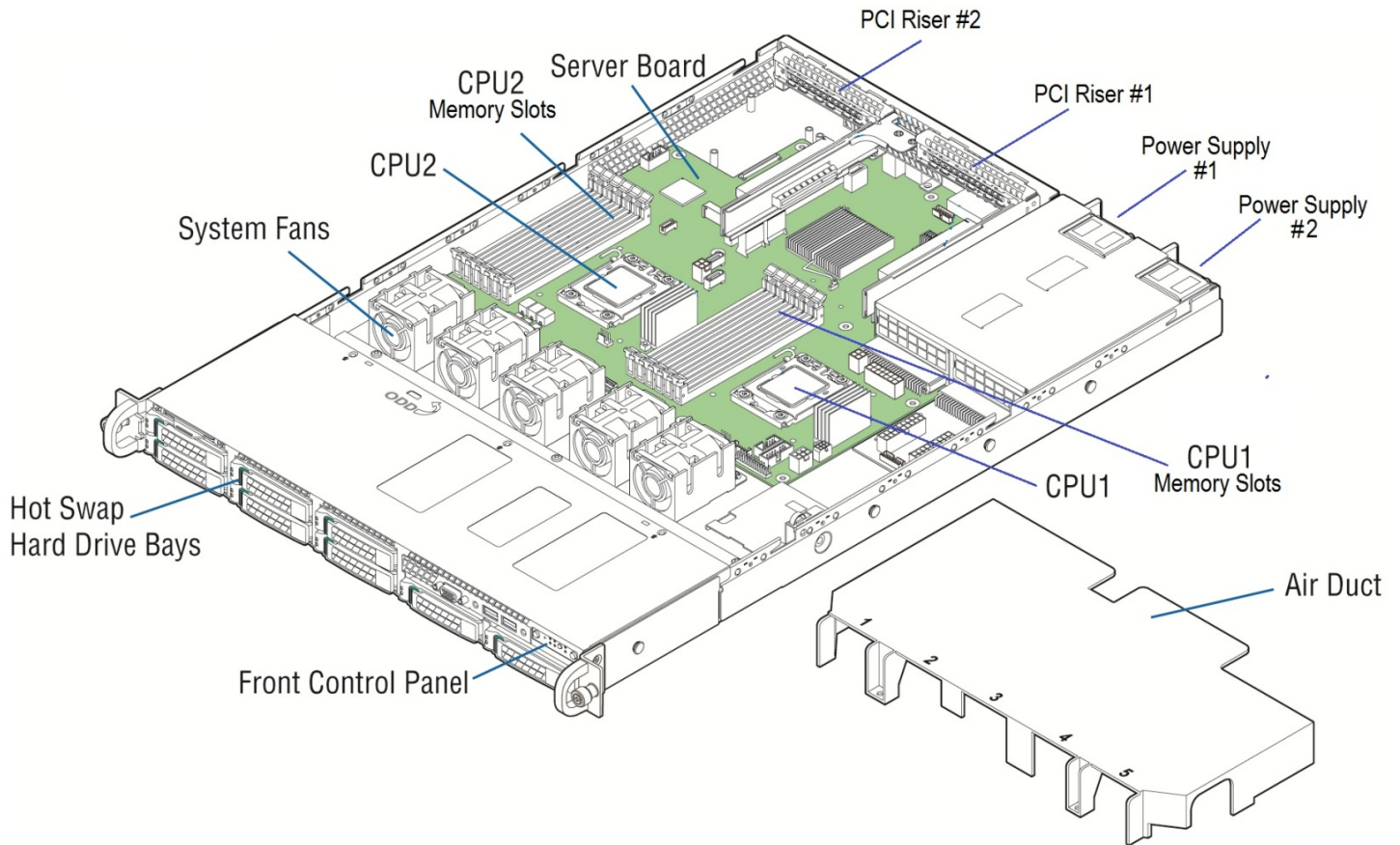
Figure 35. Intel® Server System R1000BB
