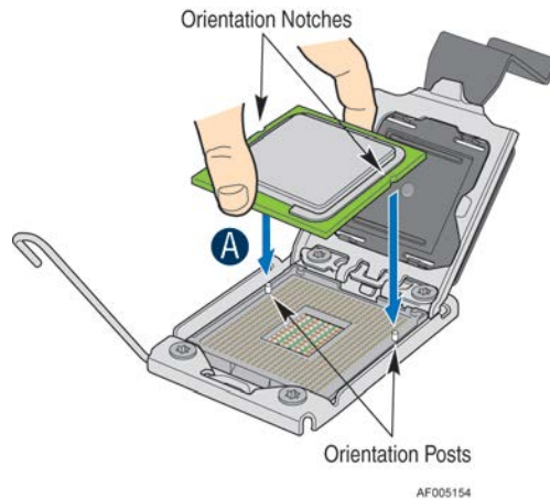
Figure 8. Processor Installation
