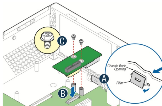
Figure 28. Intel® RMM4 Dedicated Management NIC Installation
