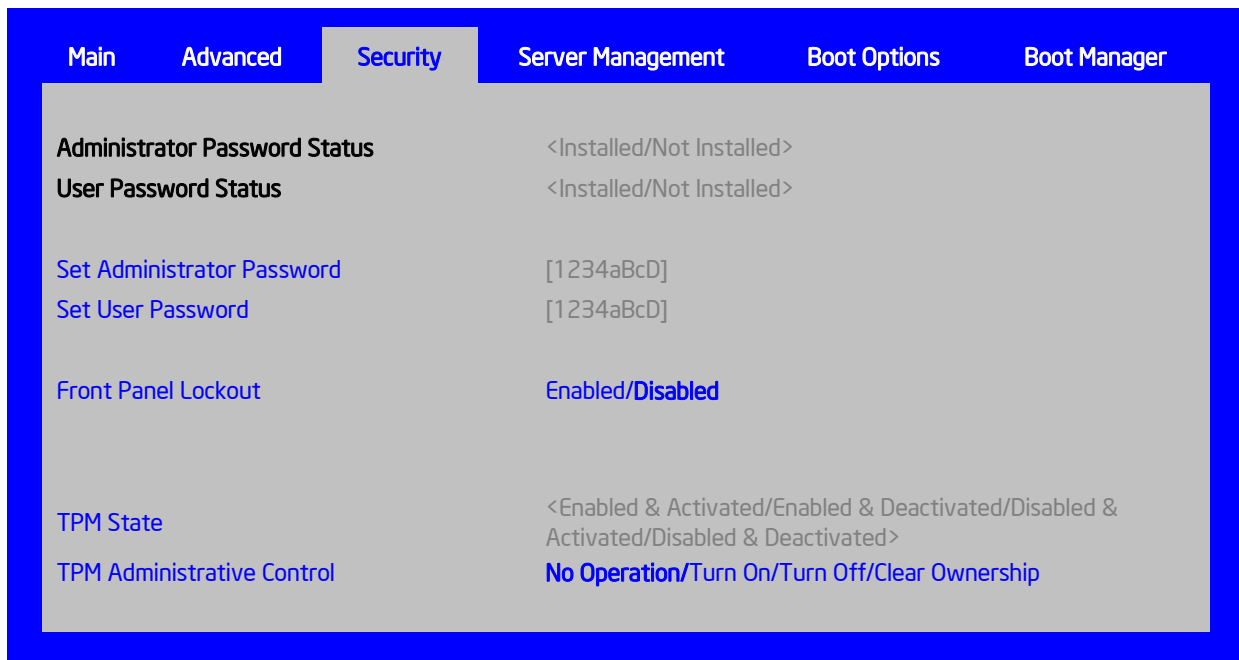
Figure 25. Setup Utility – TPM Configuration Screen
