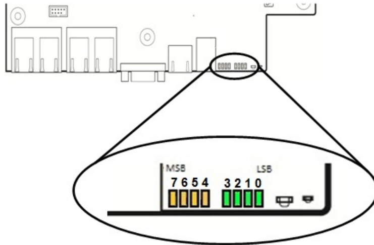
Figure 34. POST Diagnostic LED Location
