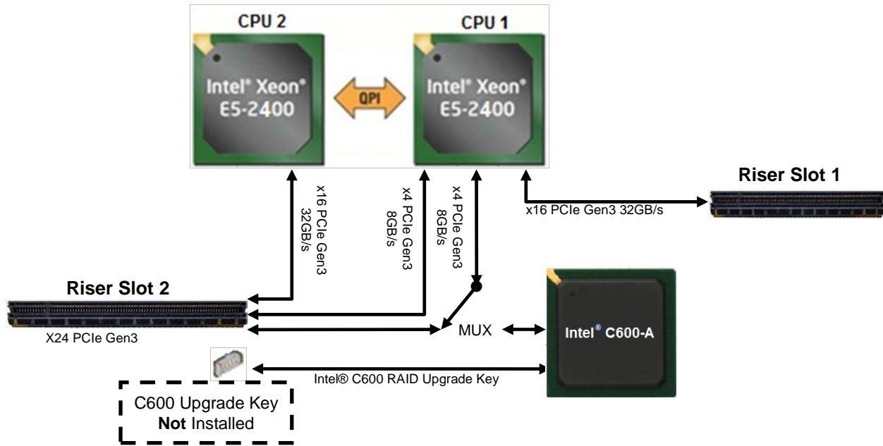
Figure 13. Riser Slot Architecture - Intel® C600 Upgrade Key NOT Installed
