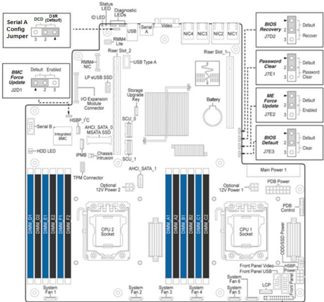
Figure 4. Jumper Block Identification
