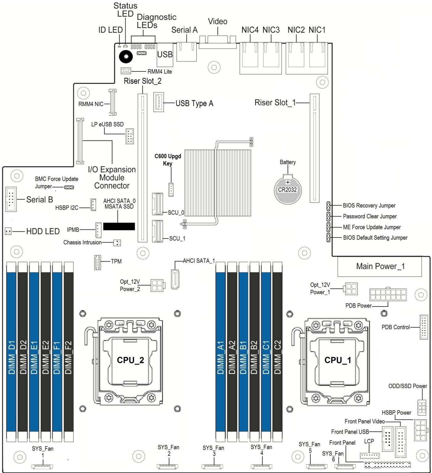
Figure 2. Server Board Component / Features Identification
