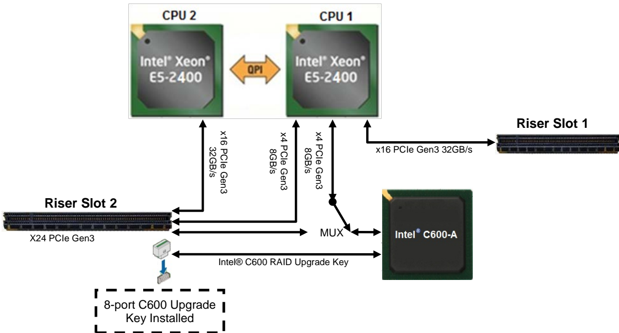
Figure 14. Riser Slot Architecture - Intel® C600 Upgrade Key Installed
