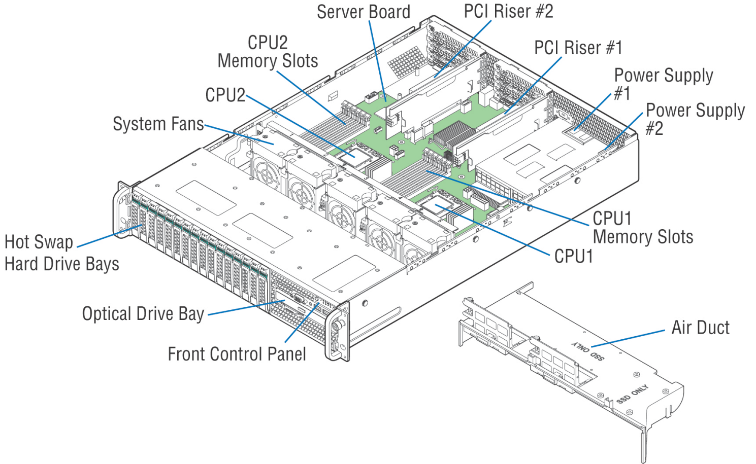
Figure 36. Intel® Server System R2000BB
