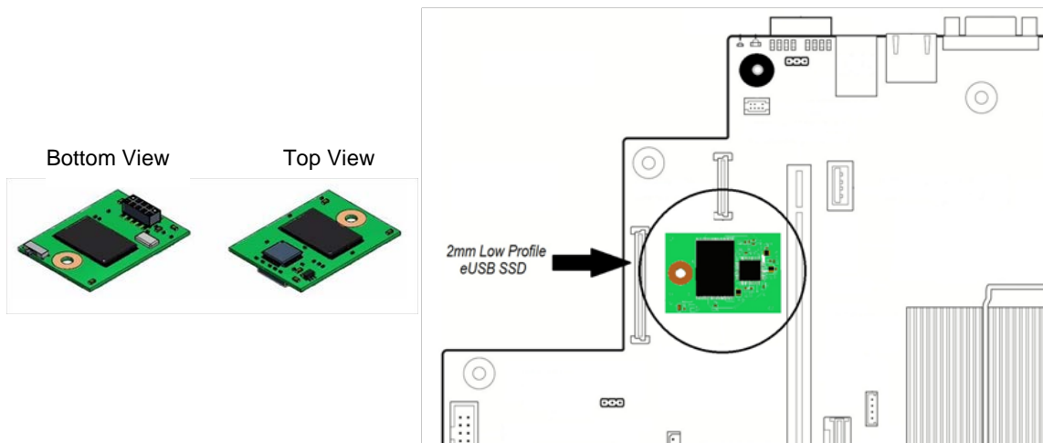
Figure 18. Low Profile eUSB SSD Support
