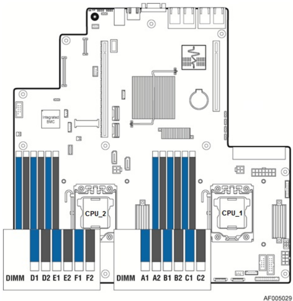
Figure 10. Intel® Server Board S2400BB Memory Slot Layout
