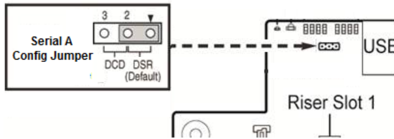
Figure 29. Serial A Configuration Jumper Block Location
