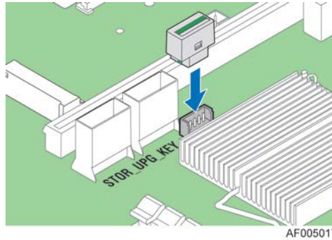
Figure 23. Intel® RAID C600 Upgrade Key Connector
