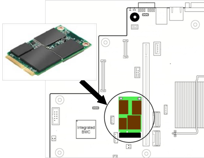
Figure 21. mSATA SSD Support
