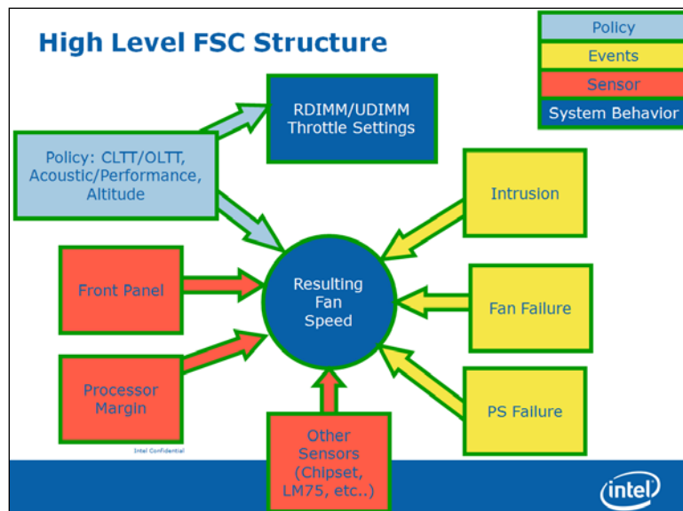
Figure 26. Fan Speed Control Process
