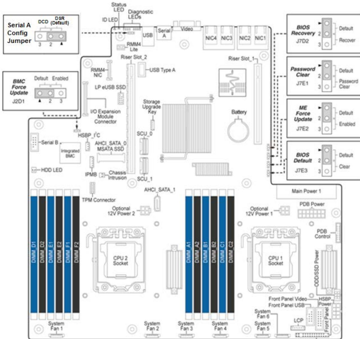
Figure 30. Reset and Recovery Jumper Block Location
