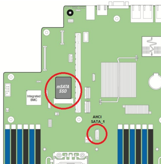
Figure 19. ACHI SATA Ports
