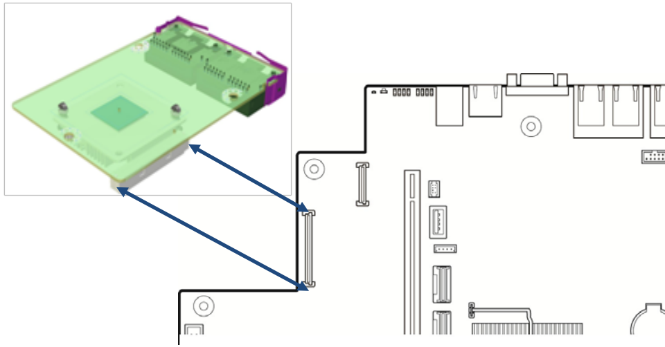
Figure 16. Server Board Layout - I/O Module Connector
