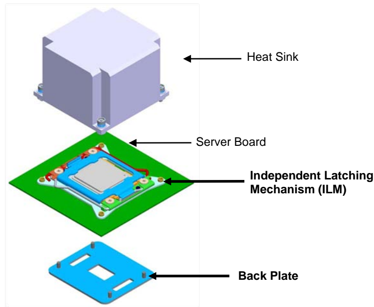
Figure 7. Processor Socket Assembly
