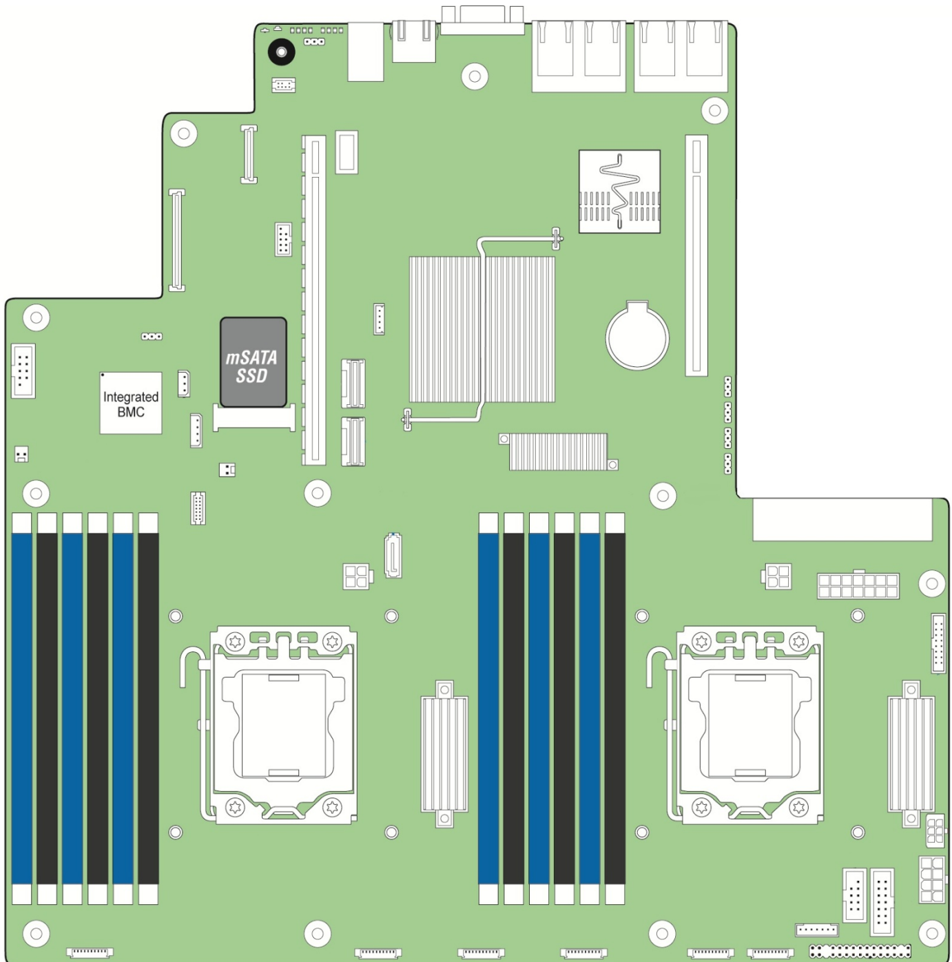
Figure 1. Intel® Server Board S2400BB
