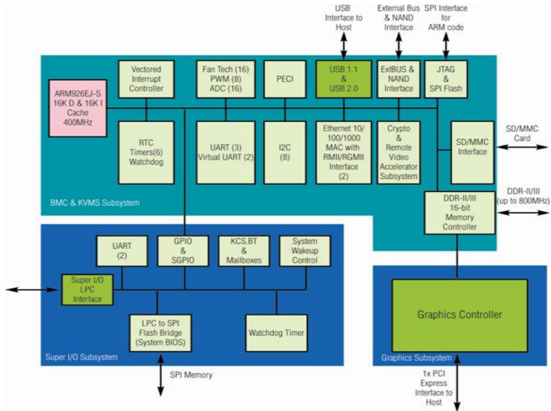
Figure 24. Integrated BMC Functional Block Diagram
