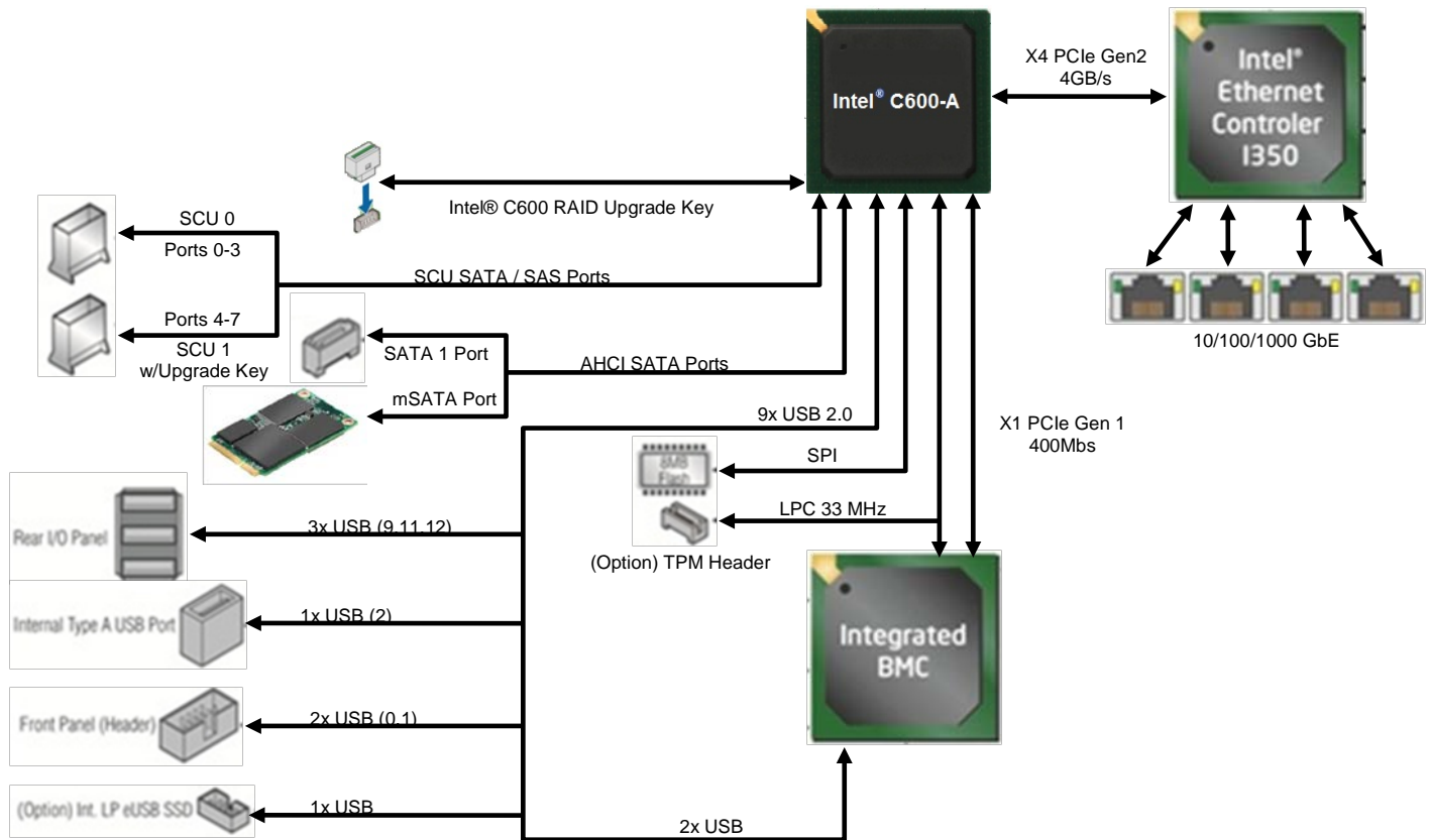
Figure 17. Functional Block Diagram - Chipset Supported Features and Functions
