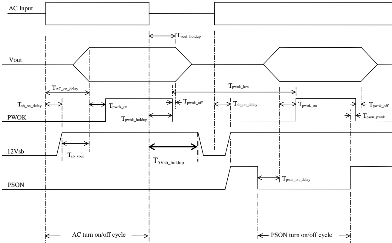
Figure 33. Turn On/Off Timing (Power Supply Signals)
