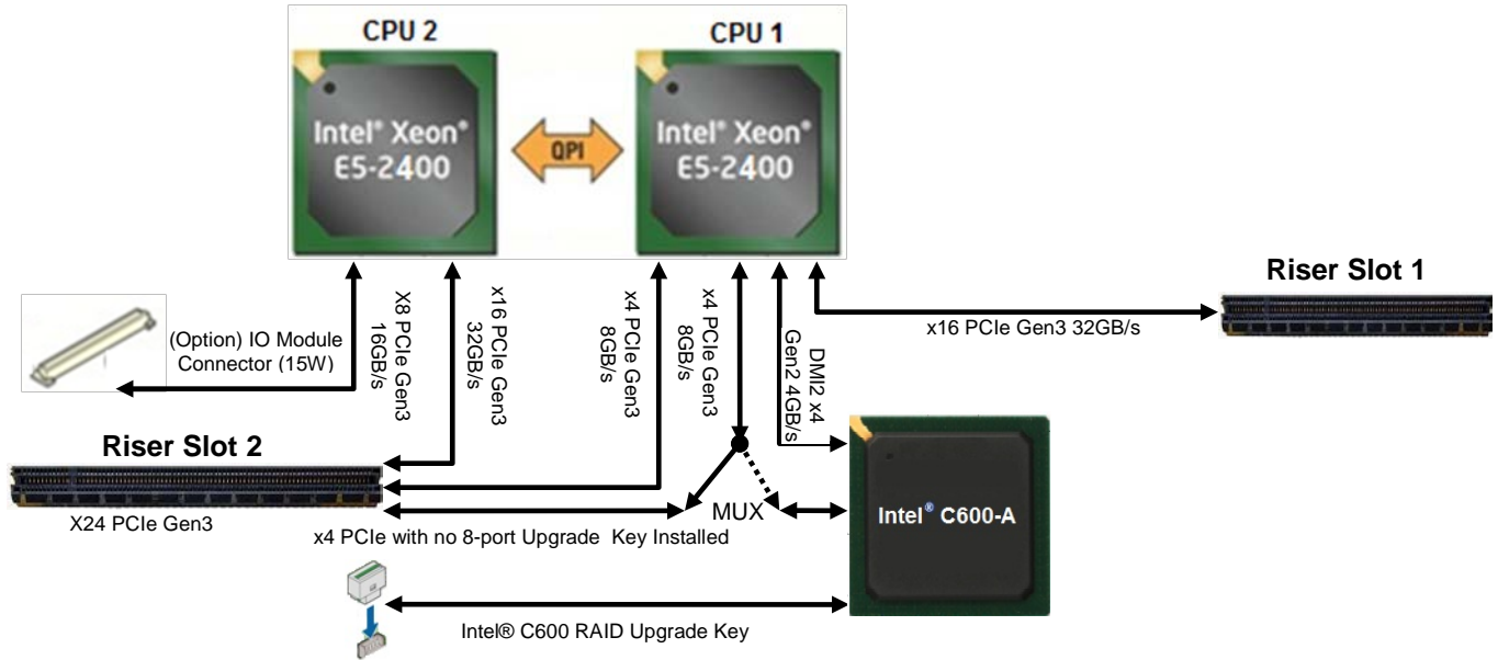
Figure 12. Processor I/O Feature Interconnect Block Diagram
