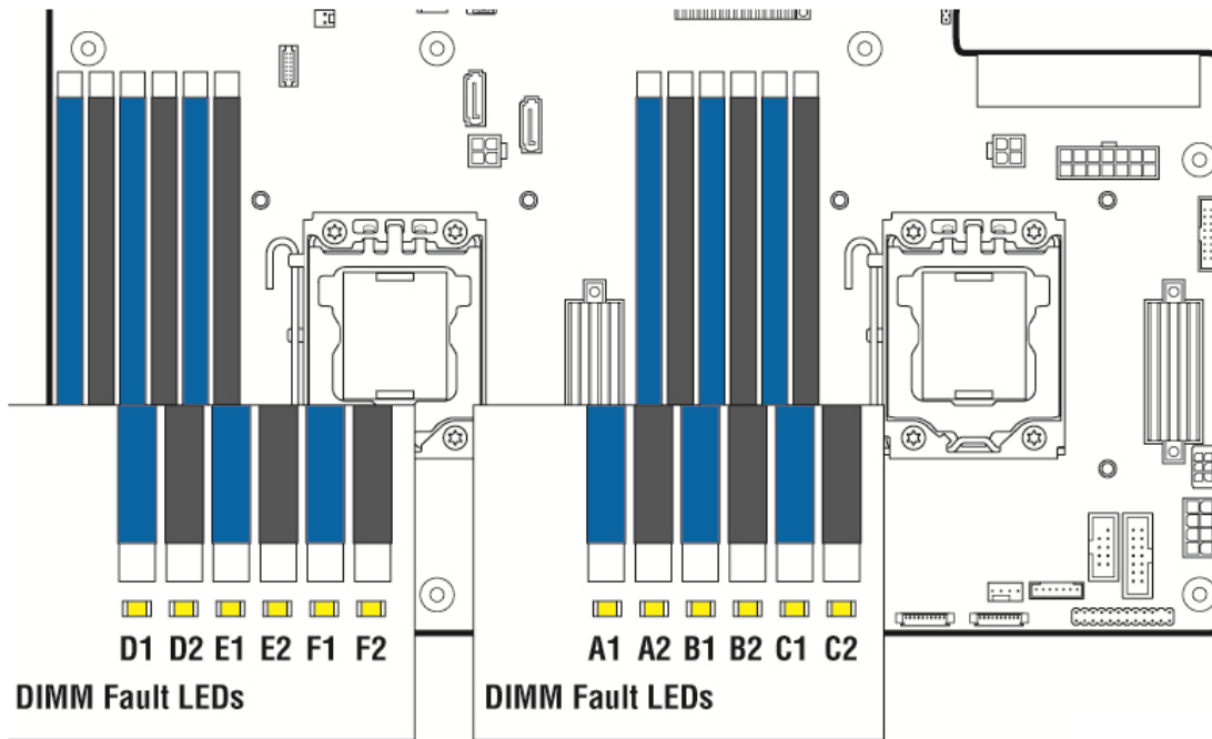
Figure 32. Memory Slot Fault LED Locations
