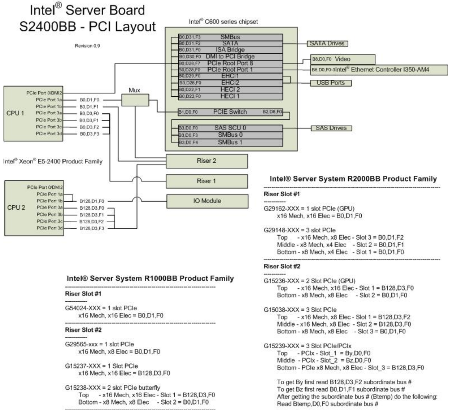
Figure 15. Intel® Server Board S2400BB PCI Bus Layout Diagram
