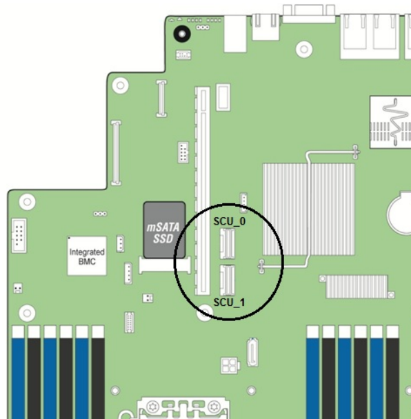
Figure 22. SCU Ports
