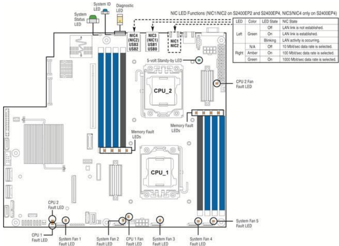
Figure 2. Intel® Light Guided Diagnostic LED Identification
