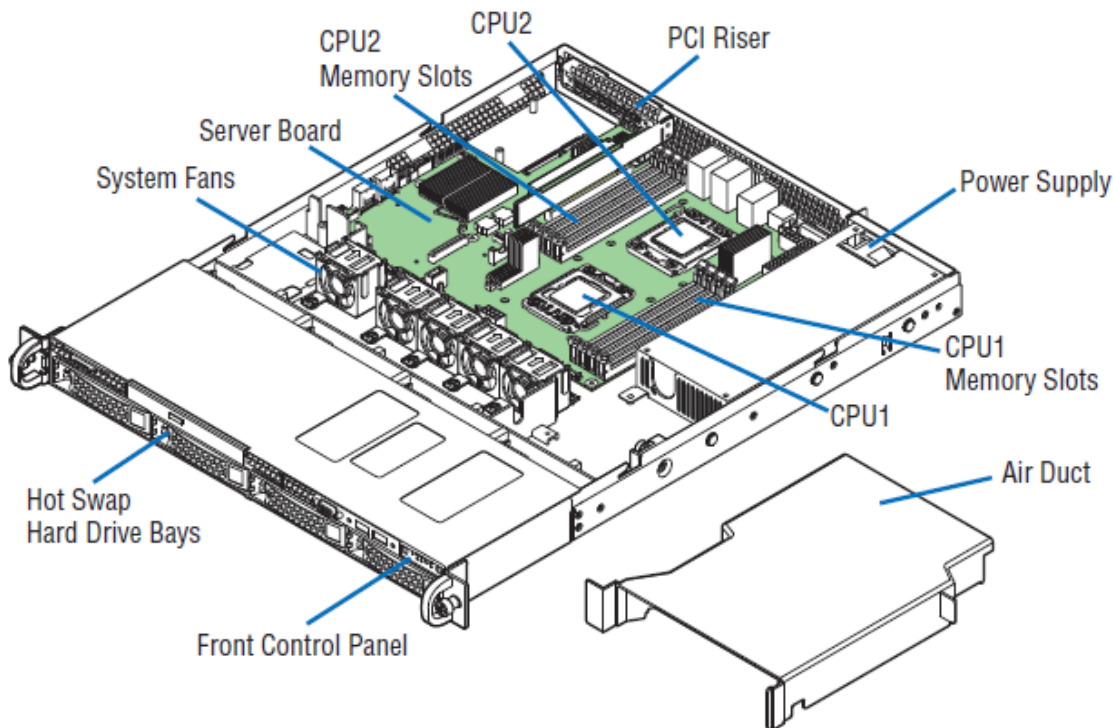
Figure 35. Intel® Server System R1000EP
