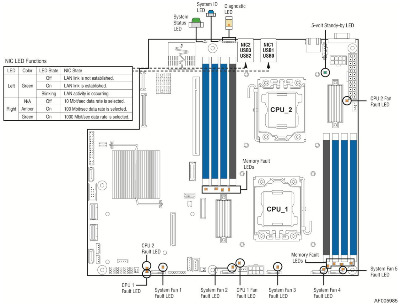
Figure 10. Intel® Light-Guided Diagnostic LEDs - Server Board
