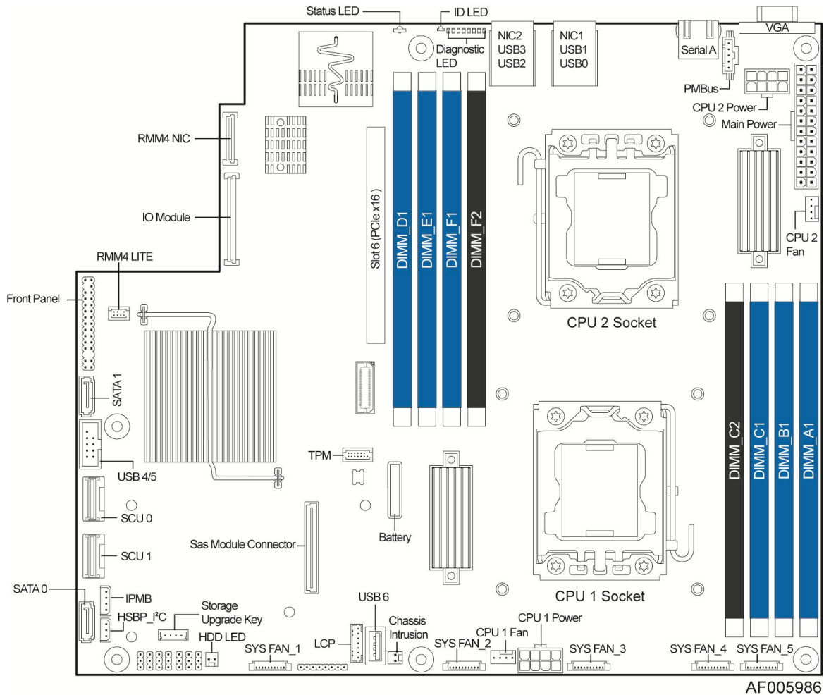
Figure 9. Intel® Server Board S2400EP
