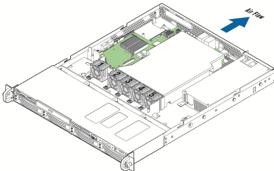
Figure 19. System Fan Identification
