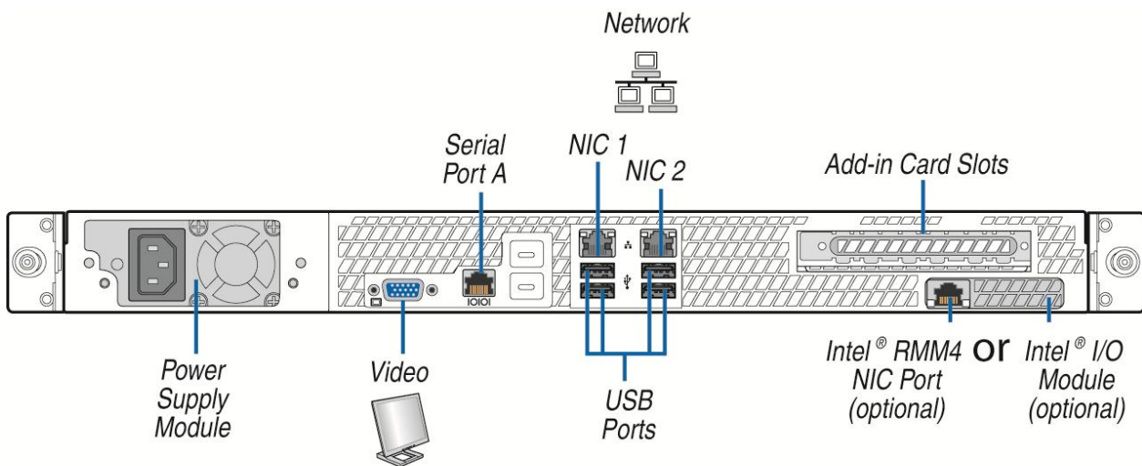
Figure 7. Back Panel Feature Identification
