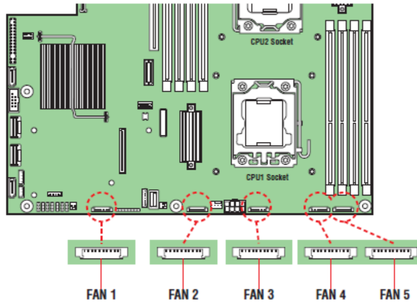
Figure 21. Intel® Server System R1000EP Server Board System Fan Connector Locations
