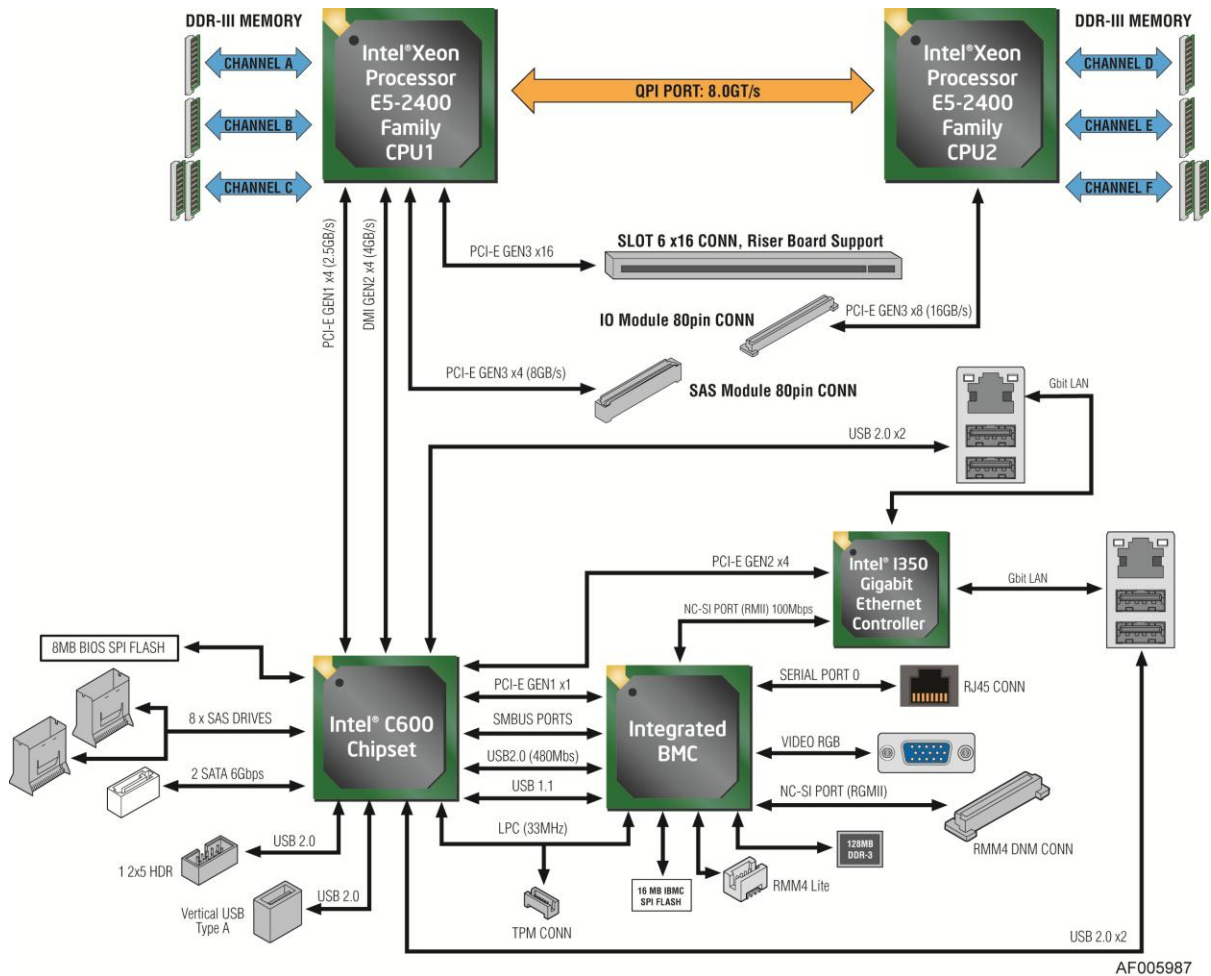
Figure 62. Riser Slot Architecture – Intel® C600 Upgrade Key NOT installed
