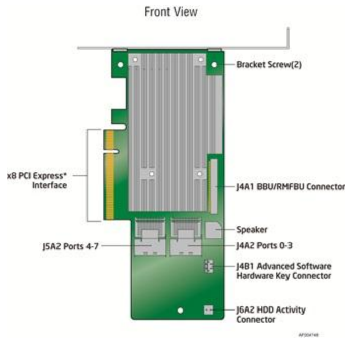
Figure 38. Intel® Integrated RAID Module RMS25PB080 and RMS25PB040
