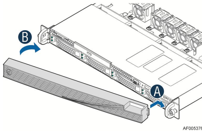
Figure 12. Installing the Optional Front Bezel
