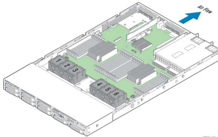
Figure 20. System Fan Identification
