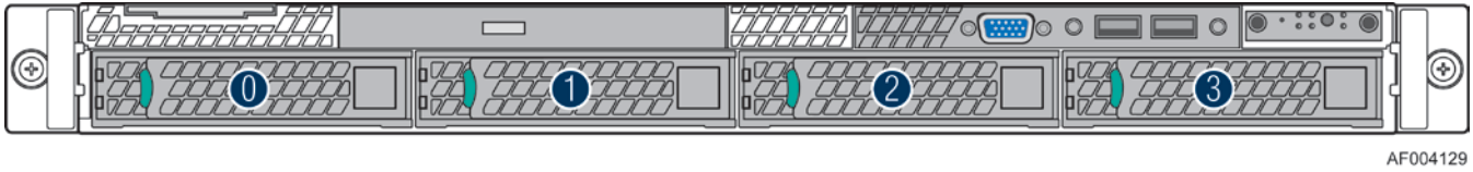
Figure 23. 3.5" Hard Drive Bay Configuration
