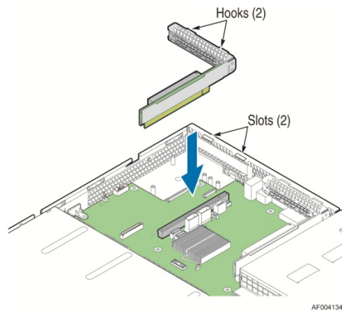
Figure 33. Add-in Card Support
