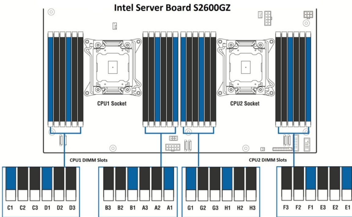
Figure 9. Intel® Server Board S2600GZ Memory Slot Layout
