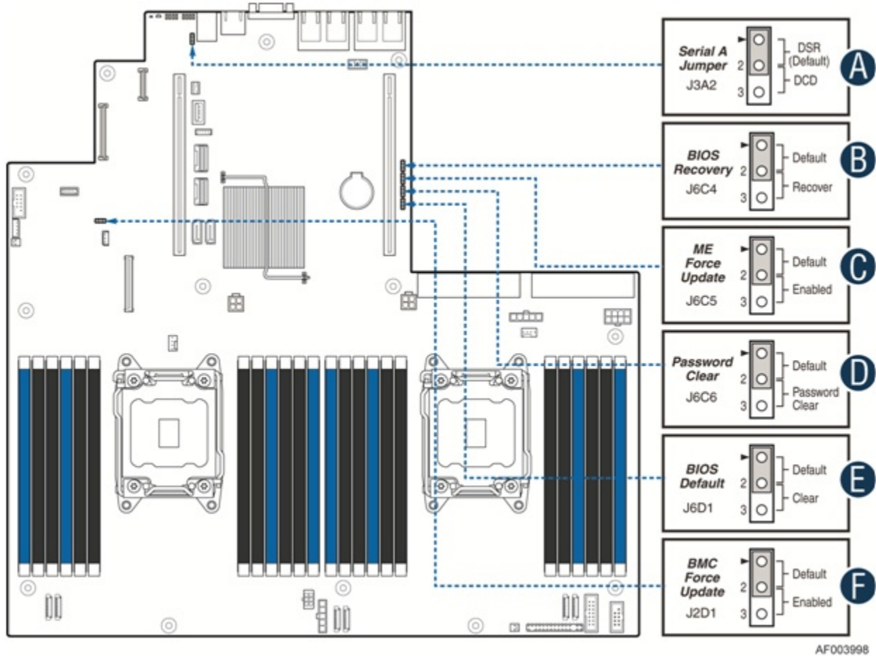
Figure 23. Reset and Recovery Jumper Block Location
