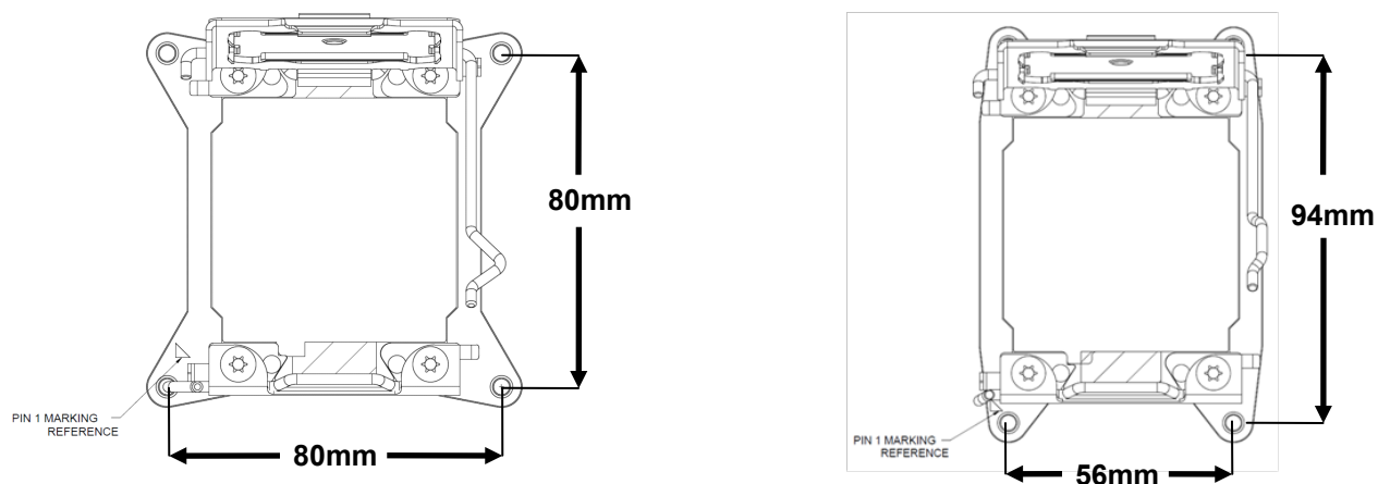
Figure 7. Processor Socket ILM Variations
