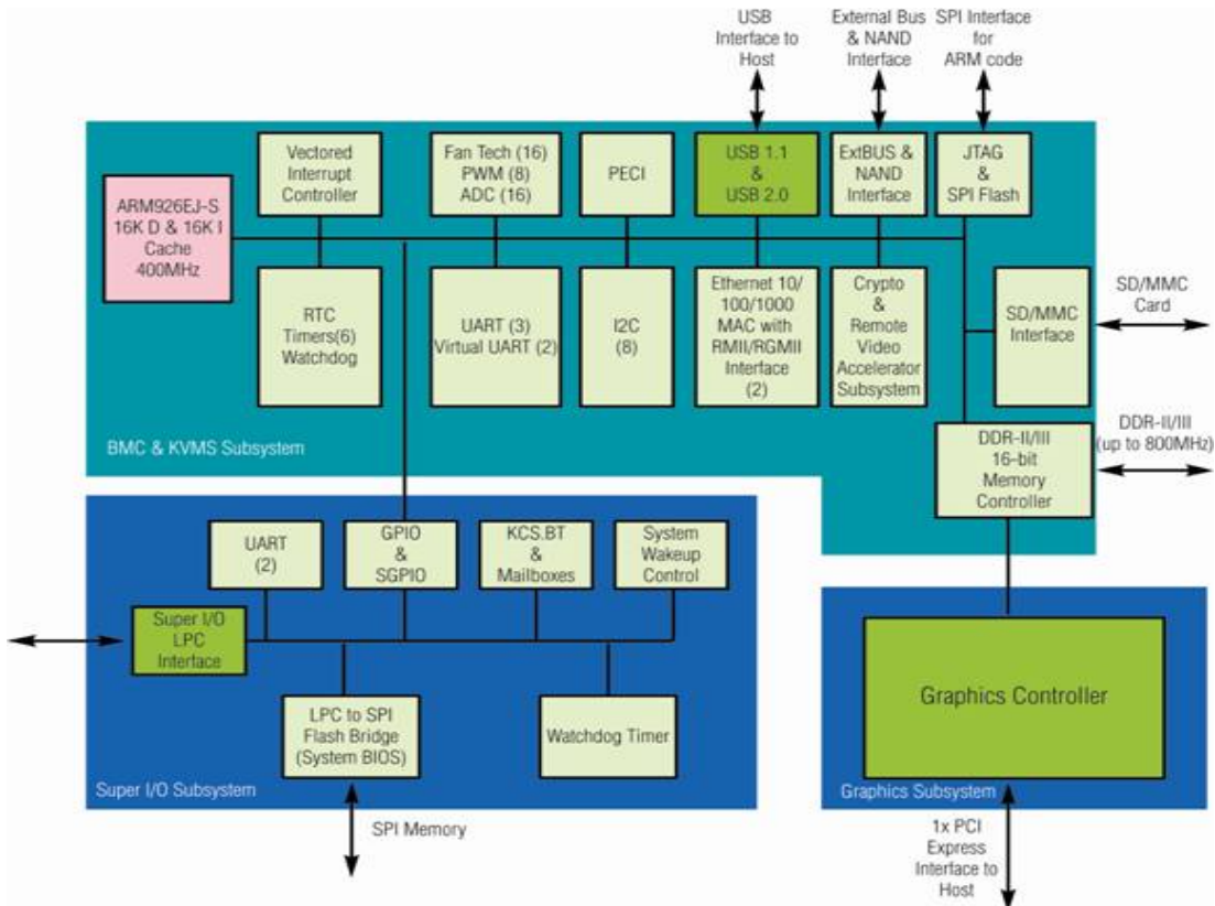
Figure 17. Integrated BMC Functional Block Diagram
