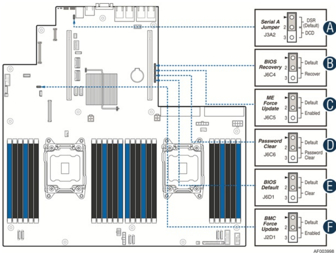
Figure 3. Jumper Block Identification
