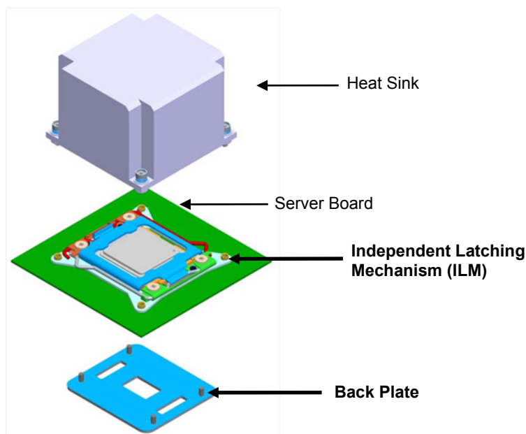
Figure 6. Processor Socket Assembly
