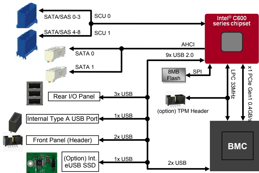
Figure 14. Functional Block Diagram - Chipset Supported Features and Functions
