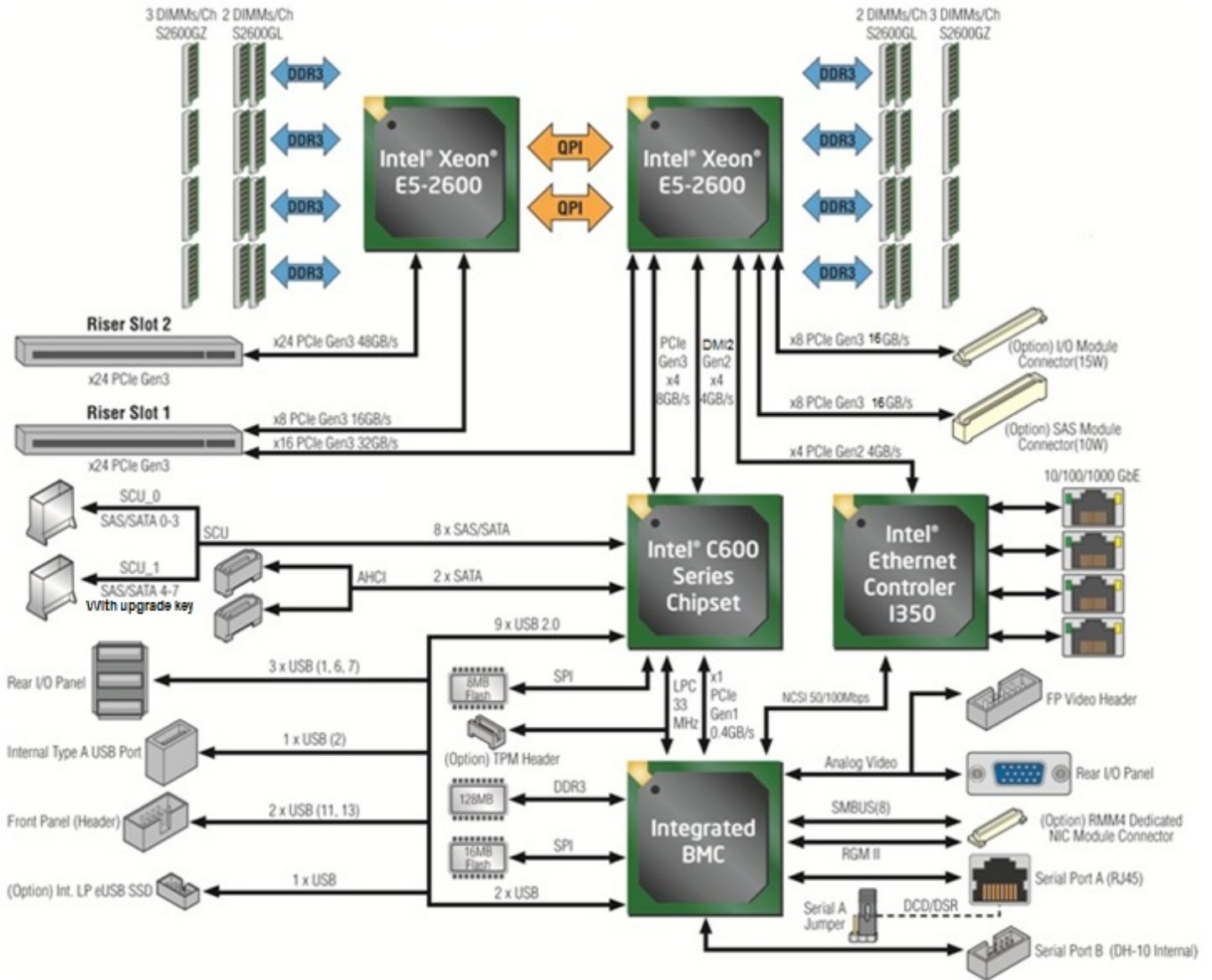
Figure 5. Intel® Server Boards S2600GZ, S2600GL Functional Block Diagram
