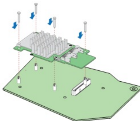
Figure 13. Server Board Layout – Intel® Integrated RAID Module Option Placement
