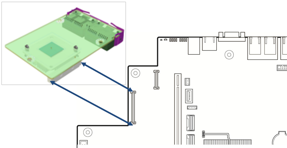
Figure 12. Server Board Layout - I/O Module Connector
