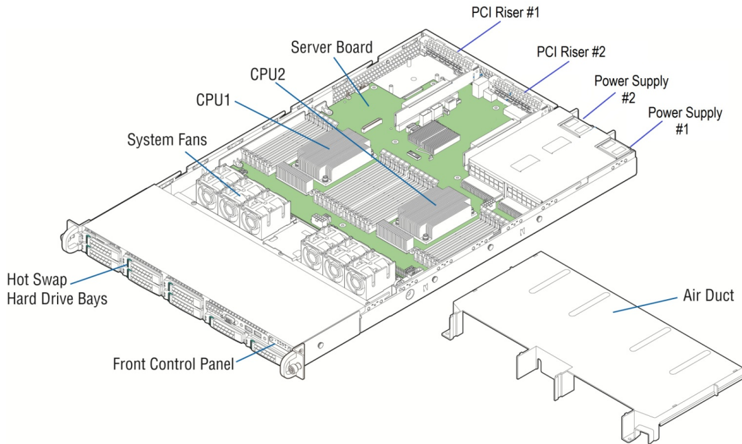
Figure 28. Intel® Server System R1000GZ/GL
