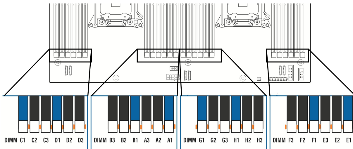
Figure 25. Memory Slot Fault LED Locations
