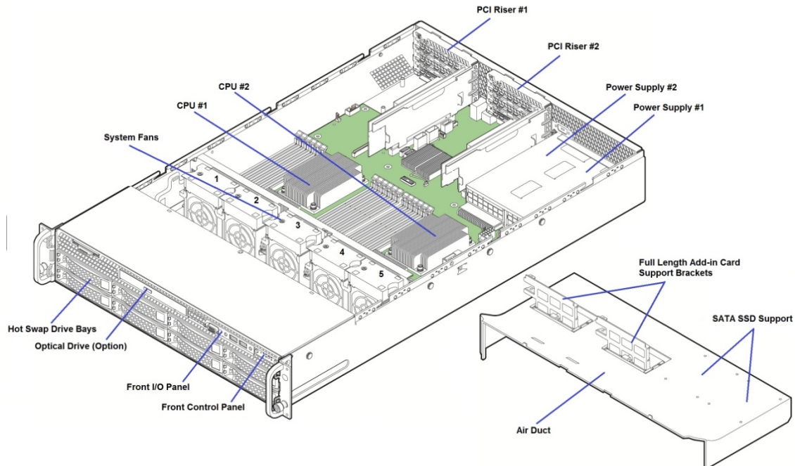
Figure 29. Intel® Server System R2000GZ/GL
