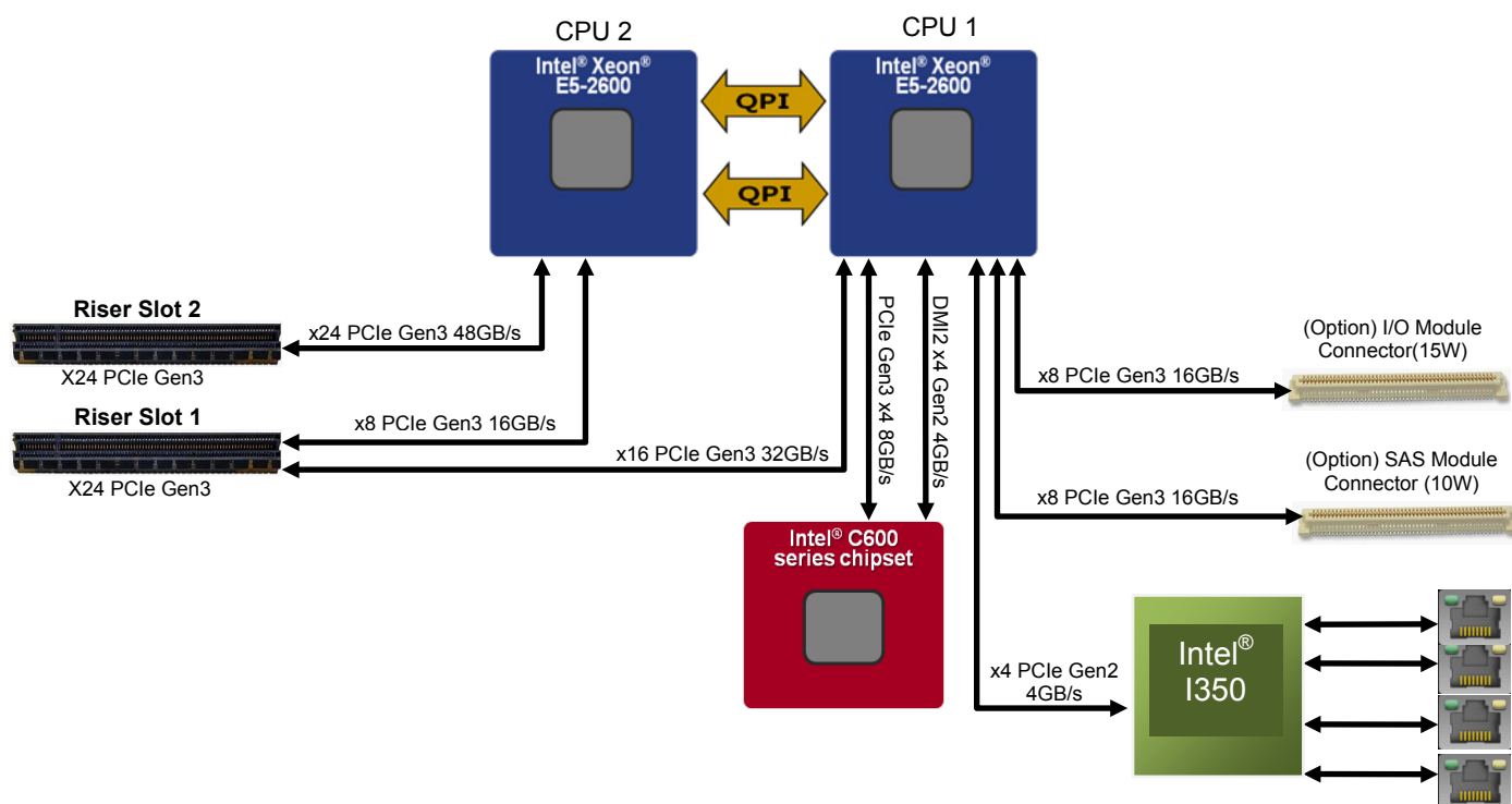
Figure 11. Functional Block Diagram of Processor IIO Sub-system
