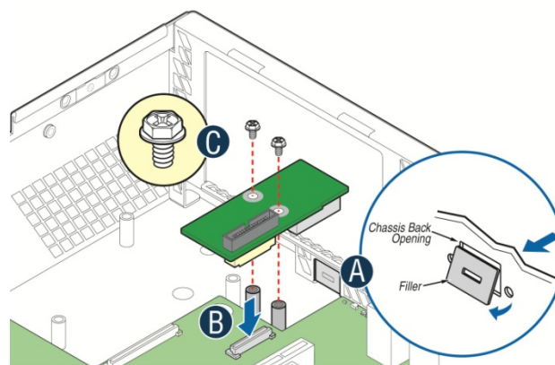
Figure 21. Intel® RMM4 Dedicated Management NIC Installation
