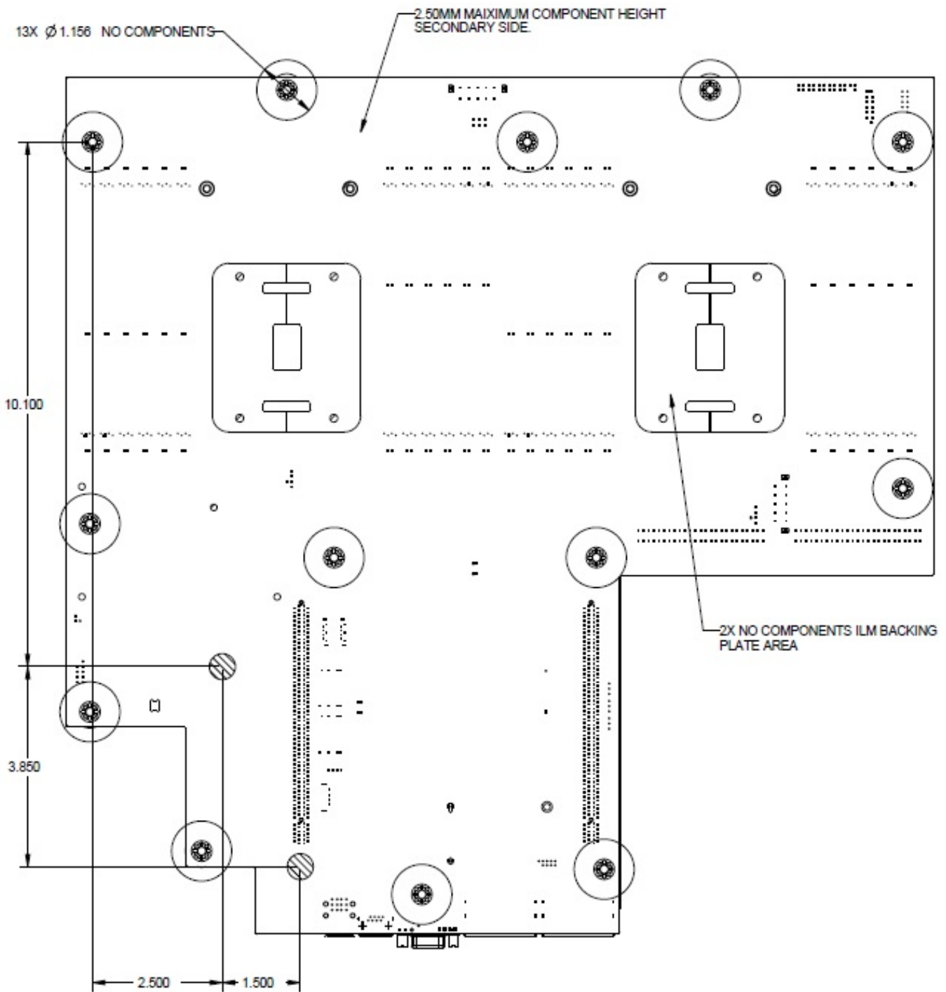
SECONDARY SIDE
