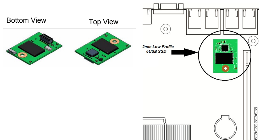
Figure 15. Low Profile eUSB SSD Support
