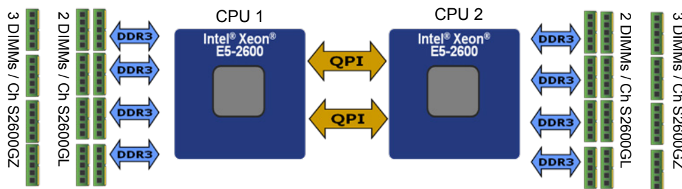
Figure 8. Integrated Memory Controller Functional Block Diagram
