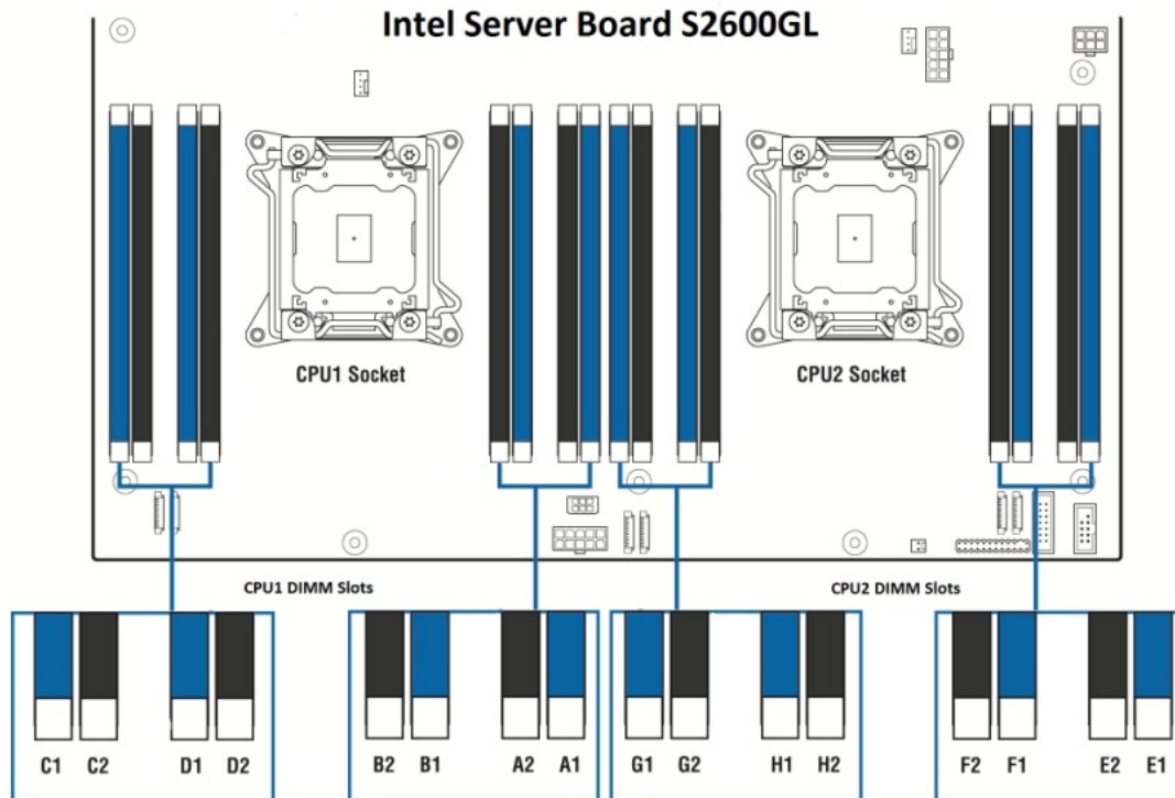
Figure 10. Intel® Server Board S2600GL Memory Slot Layout
