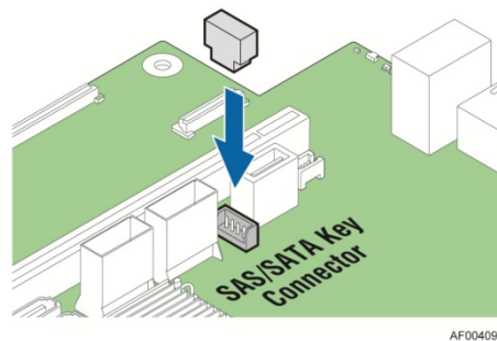
Figure 16. Intel® RAID C600 Upgrade Key Connector
