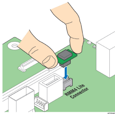
Figure 20. Intel® RMM4 Lite Activation Key Installation
