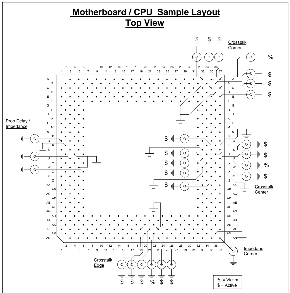
Figure 5. Socket parasitic test board layout.
