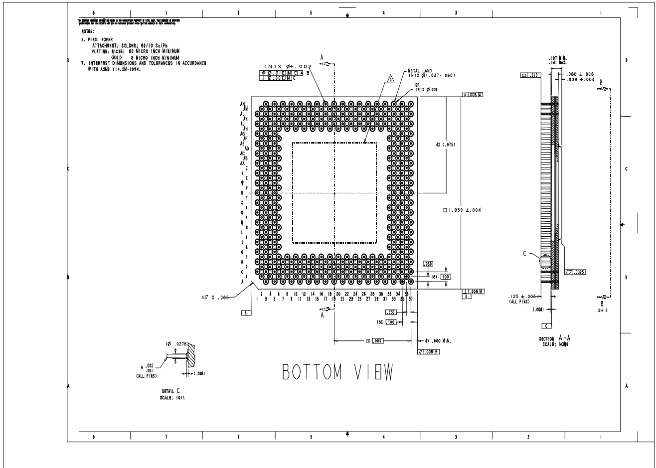
Figure 3. Outline of the processor packages that can be used with the 370-pin socket
